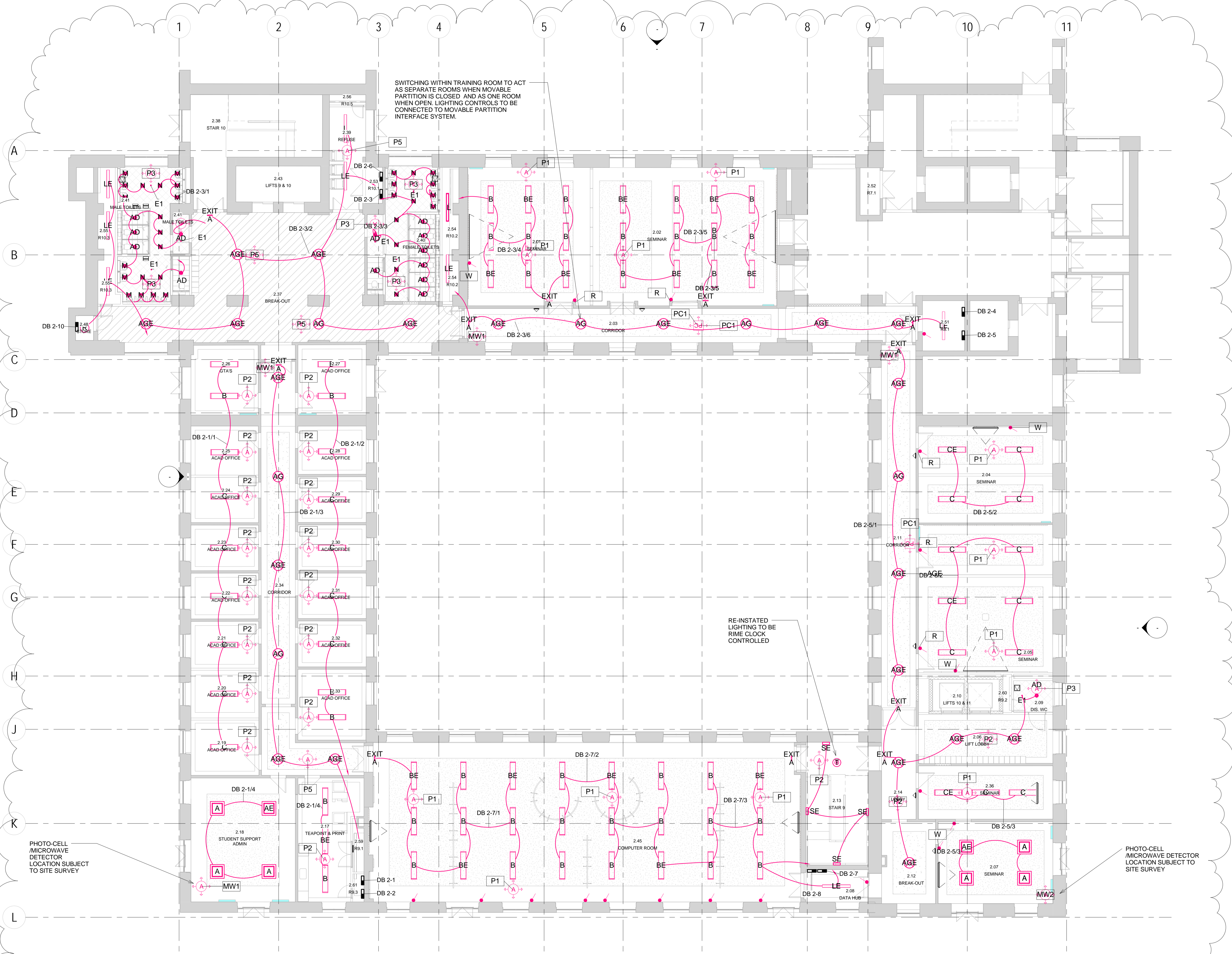
04 Second Floor - Lighting 1:100
