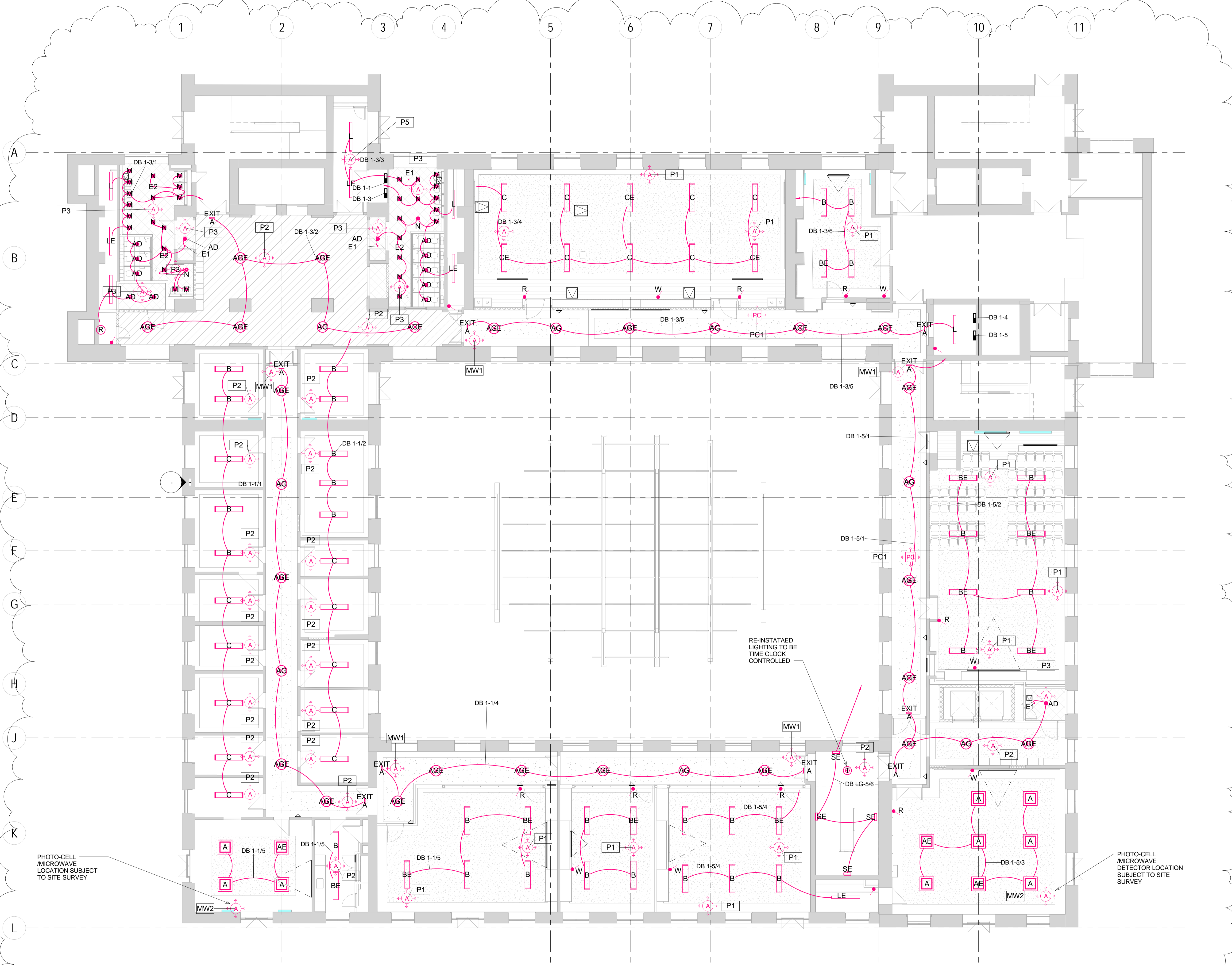
03 First Floor - Lighting 1:100
