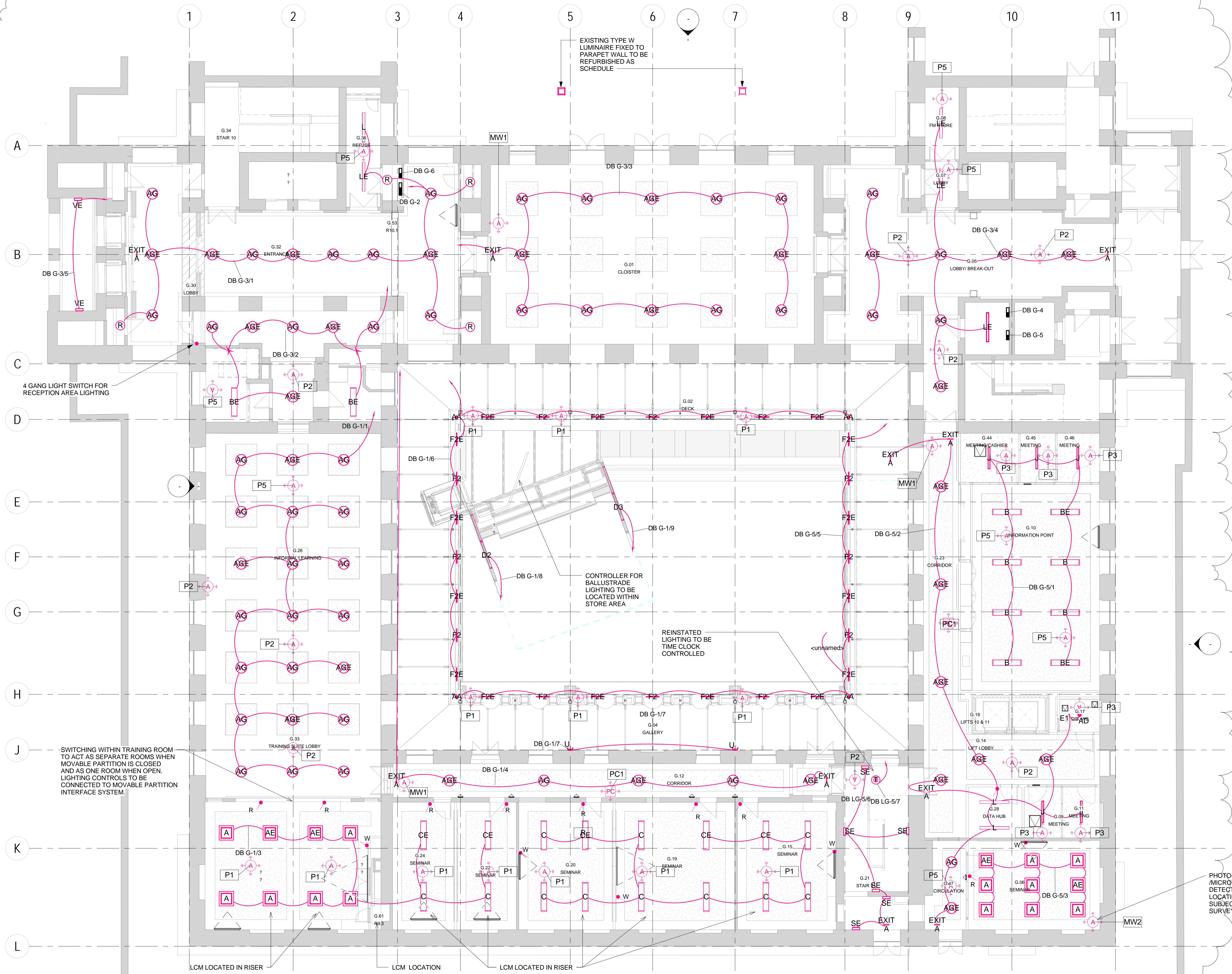
02 Ground Floor - Lighting 1:100
