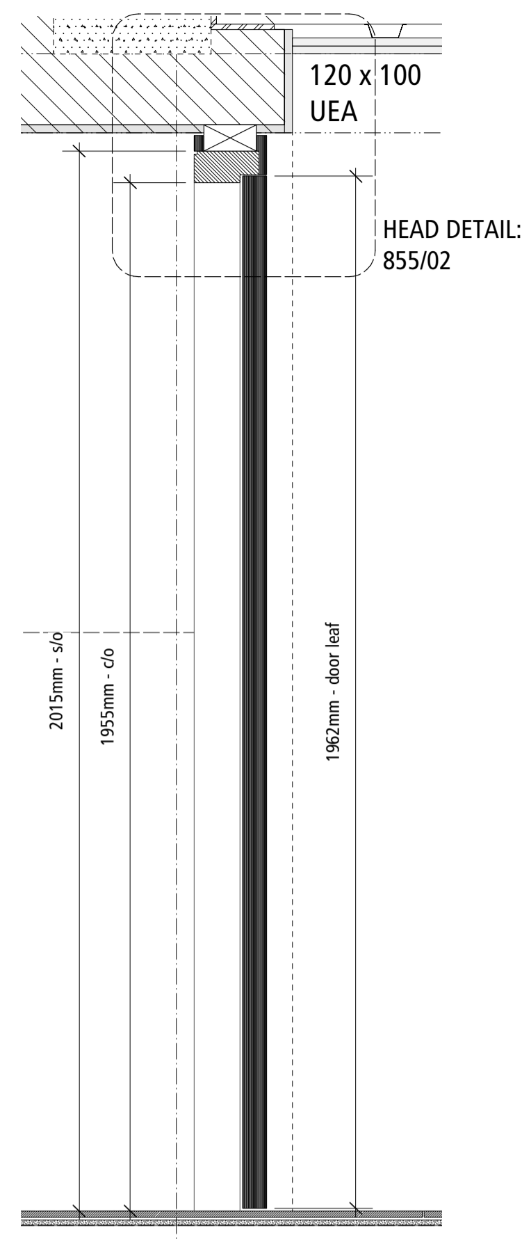
PROPOSED SECTION OF DB.08 SCREEN INFILL @ 1:10
