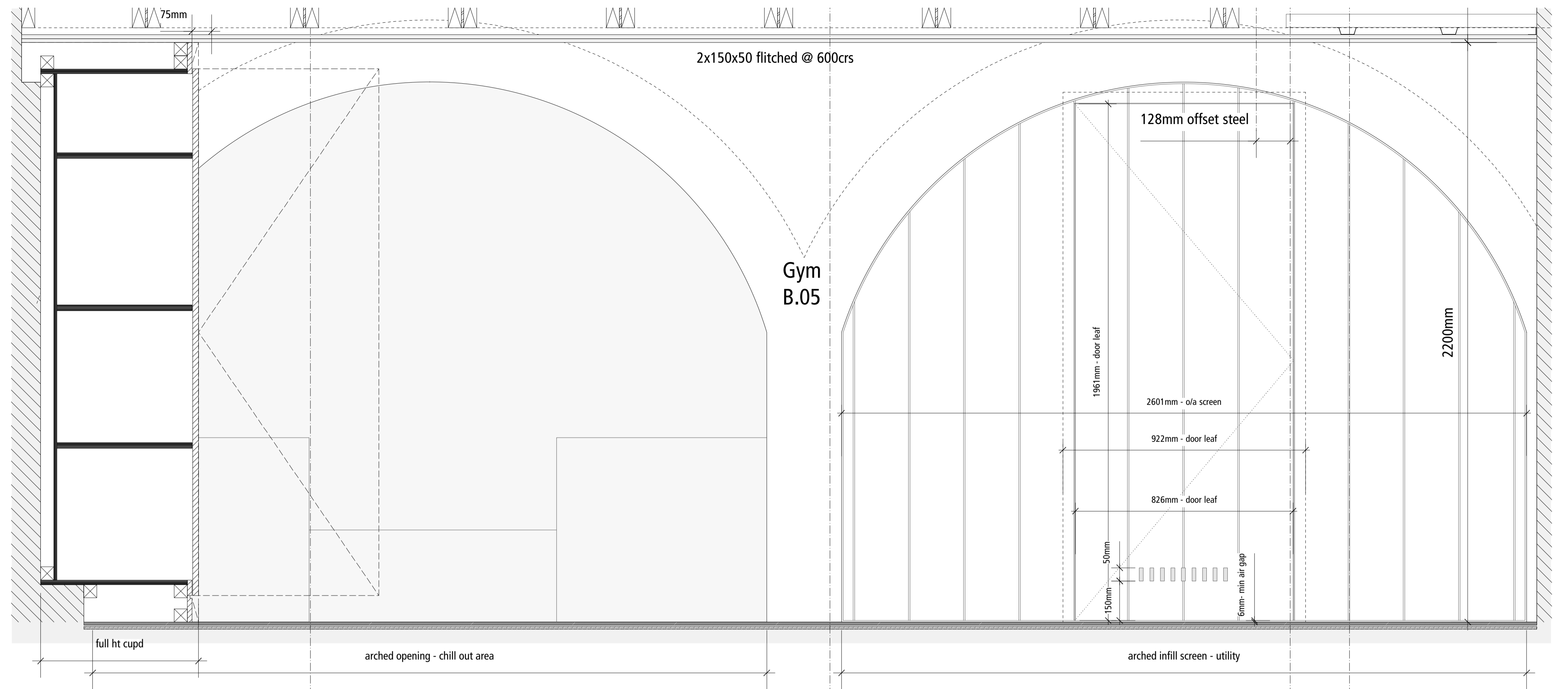
PROPOSED ELEVATION OF DB.08 SCREEN INFILL @ 1:10
