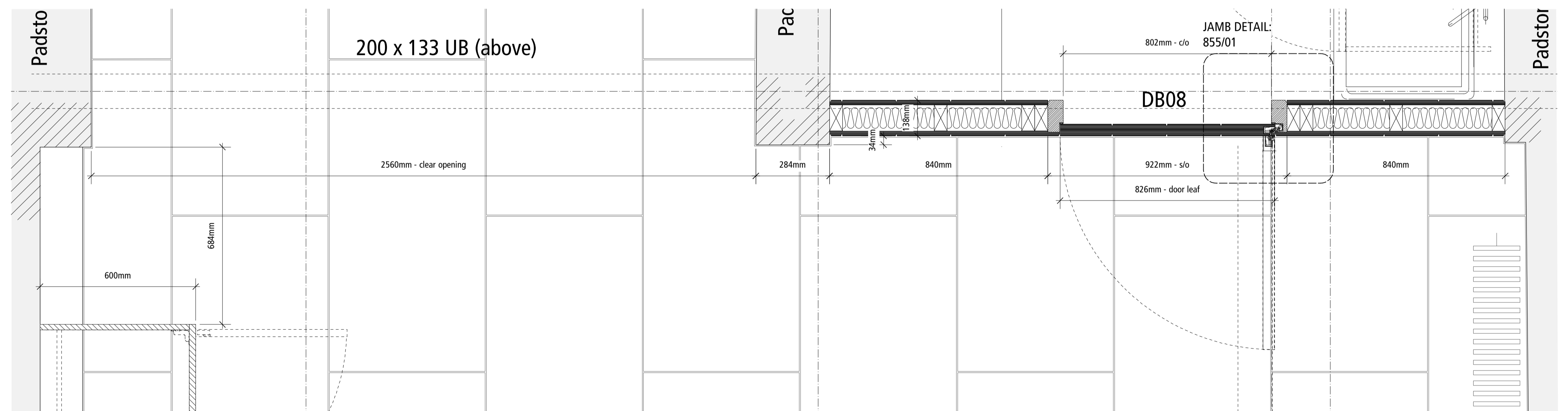
PROPOSED PLAN OF DB.08 SCREEN INFILL @ 1:10
