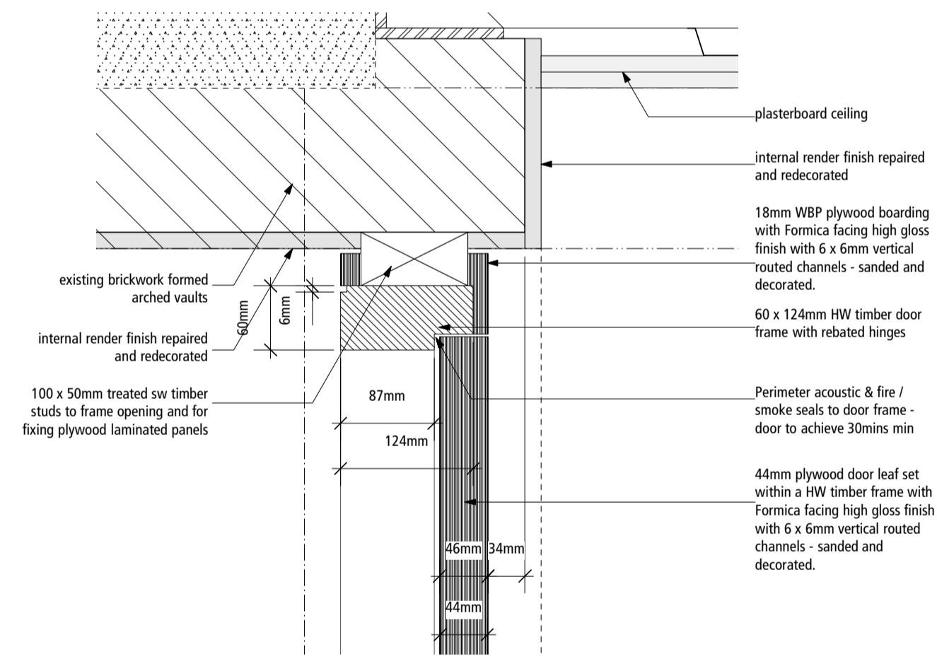
855/02 - HEAD DETAIL @ 1:5
