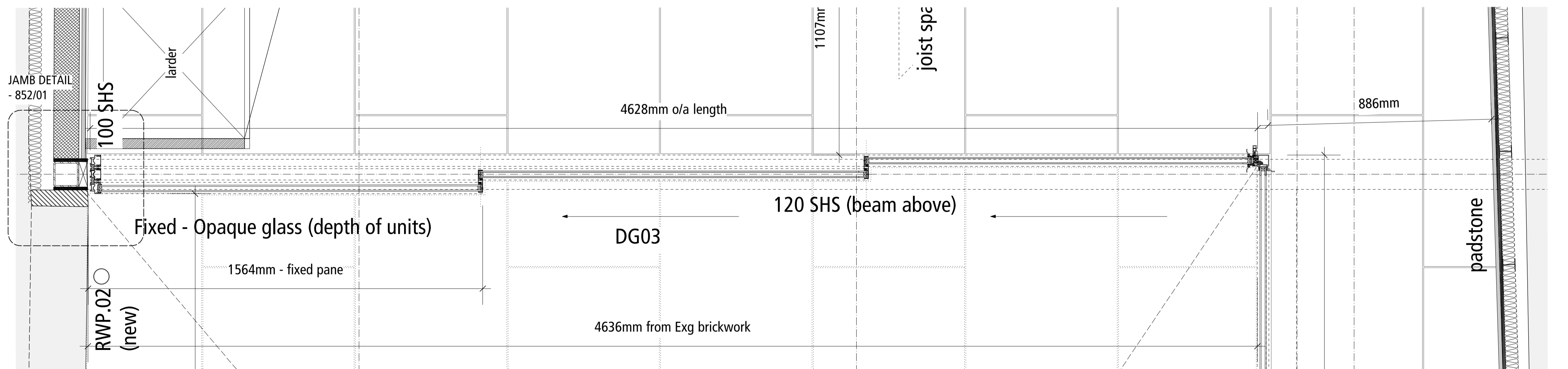
PROPOSED PLAN OF DG.03 @ 1:10
