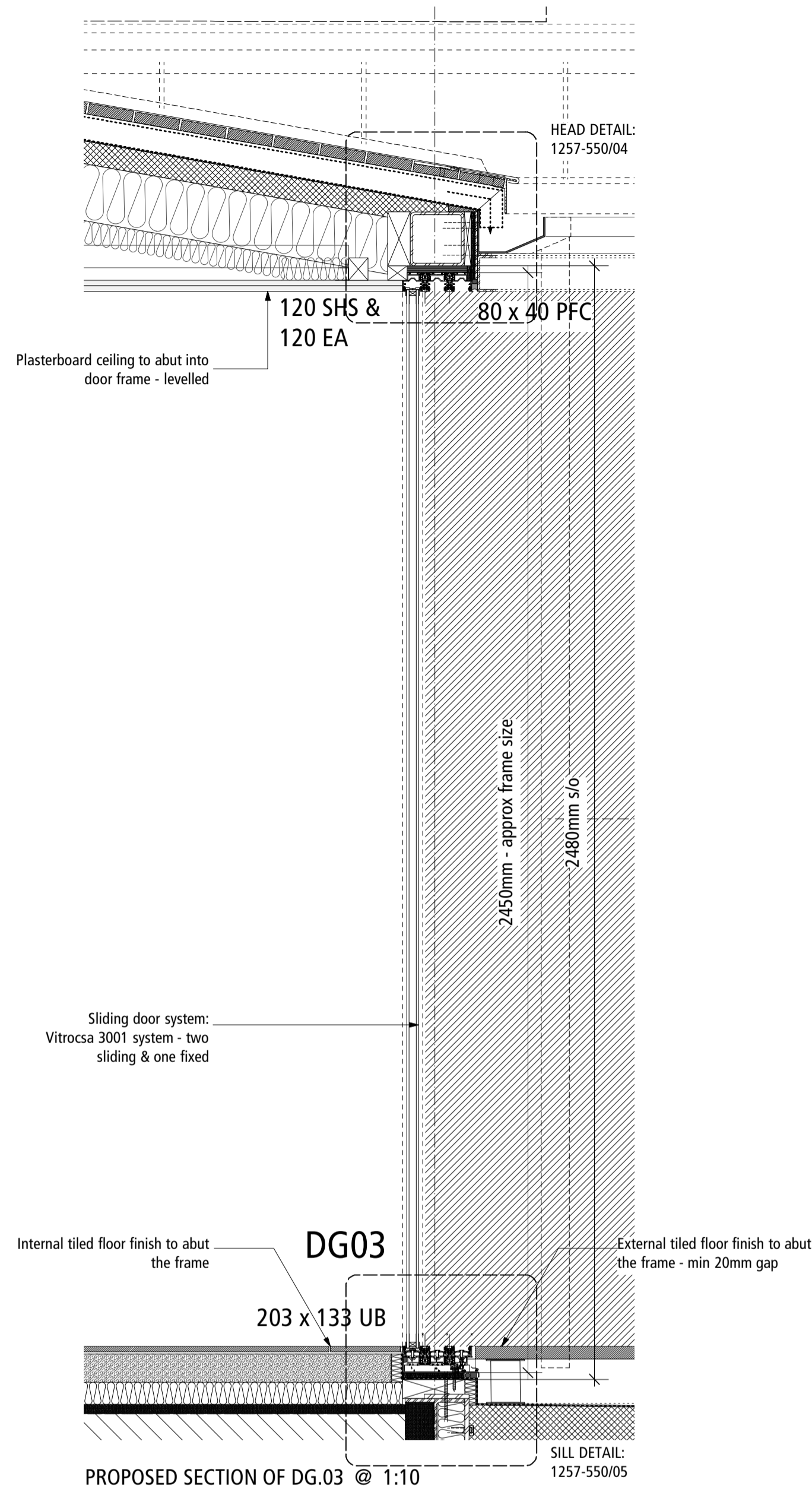
PROPOSED SECTION OF DG.03 @ 1:10
