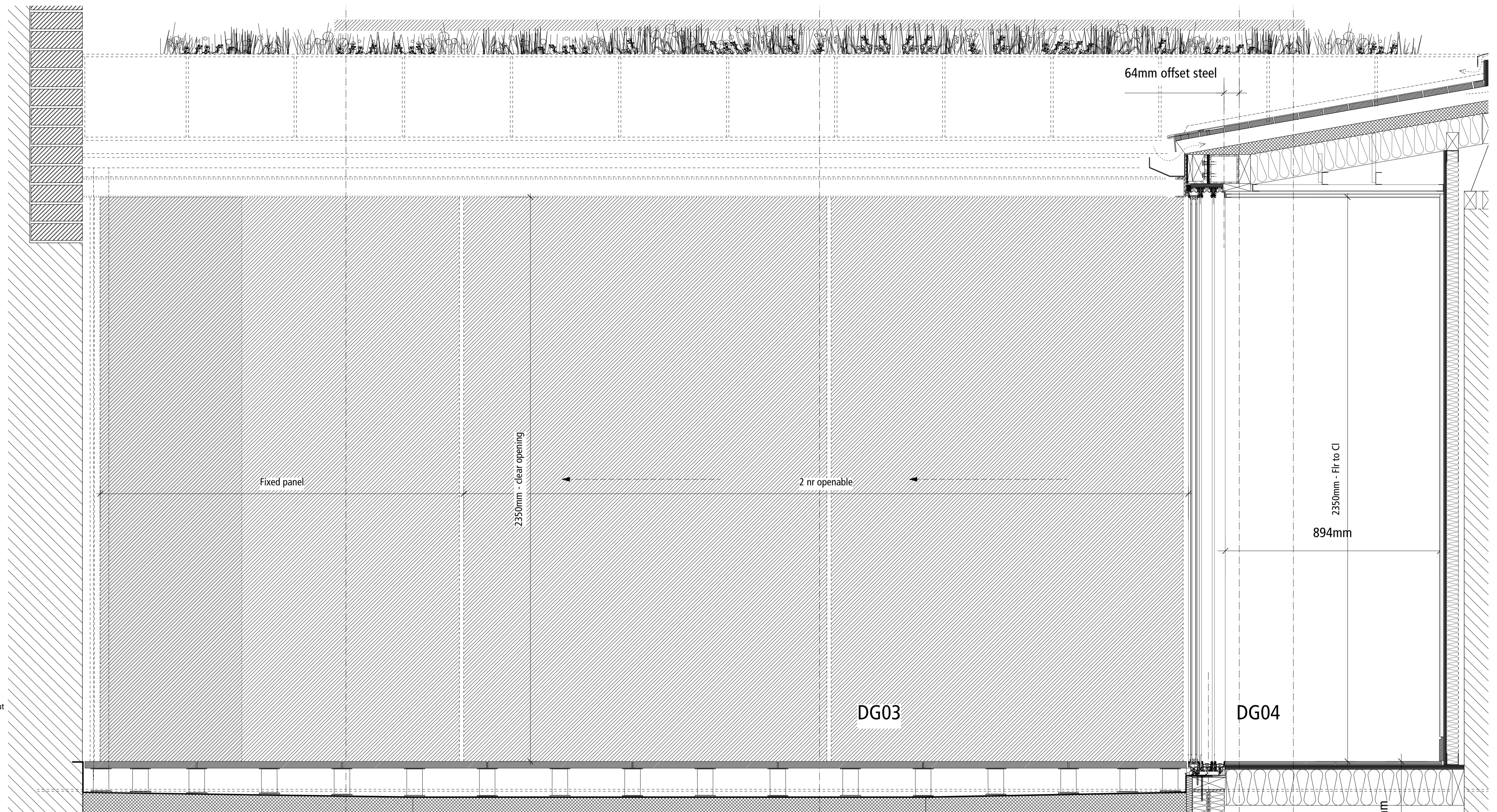
PROPOSED ELEVATION OF DG.03 @ 1:10
