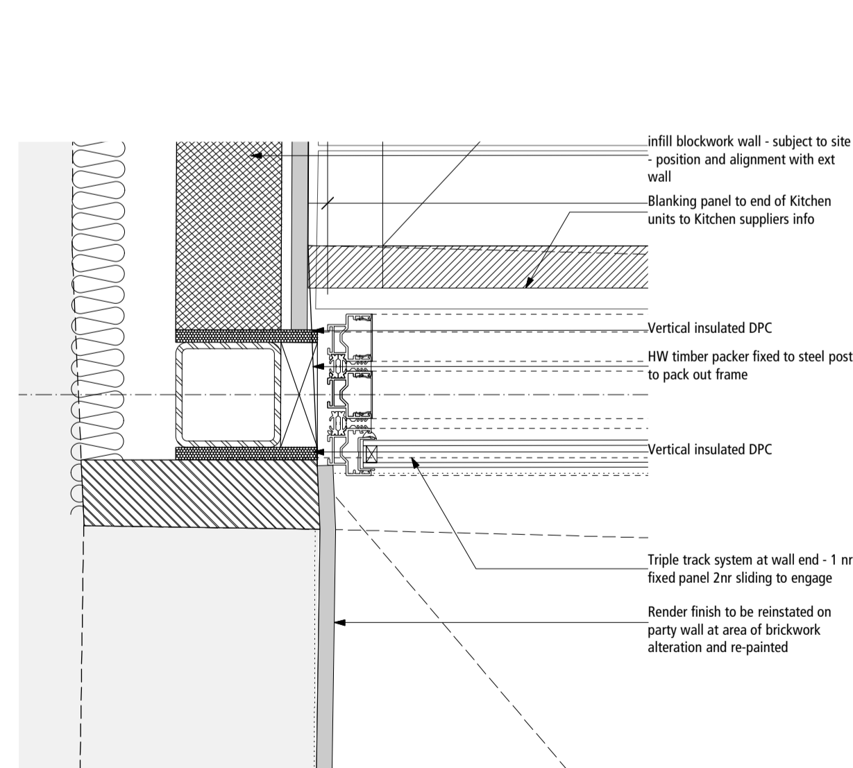
852/01 - JAMB WITH EXISTIN WALL @ 1:5
