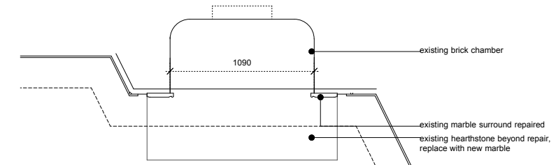
MIDDLE ROOM (G03) PART PLAN OF FIREPLACE 02 Scale 1:20@A1, 1:40@A3
