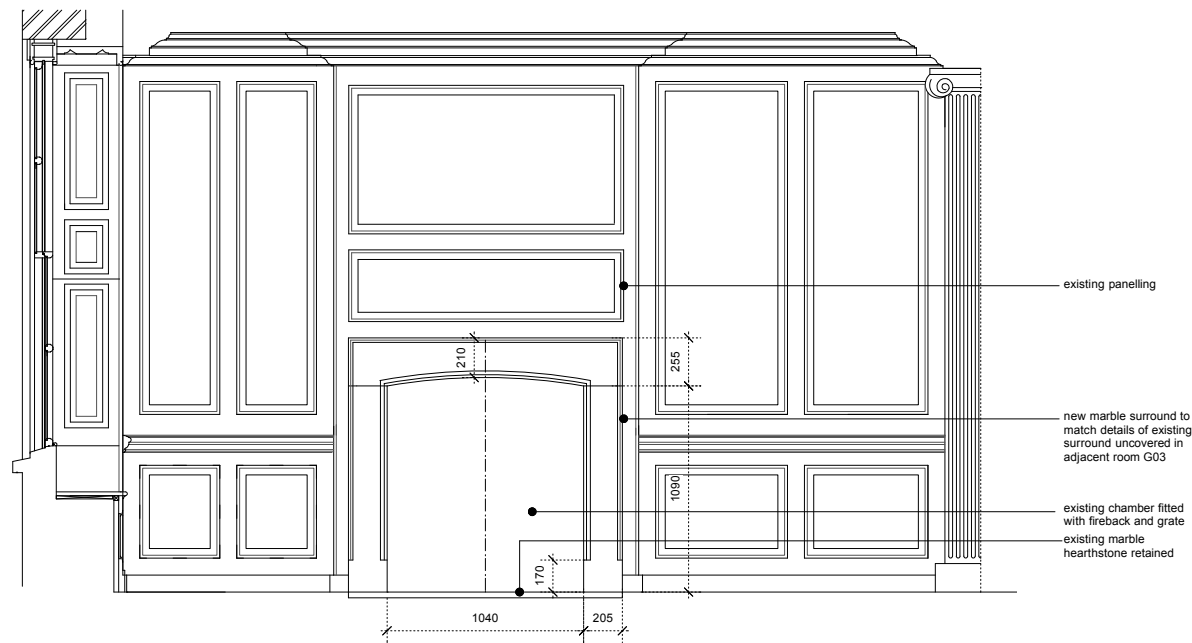
FRONT ROOM (G02) FRONT ELEVATION OF FIREPLACE 01 Scale 1:20@A1, 1:40@A3
