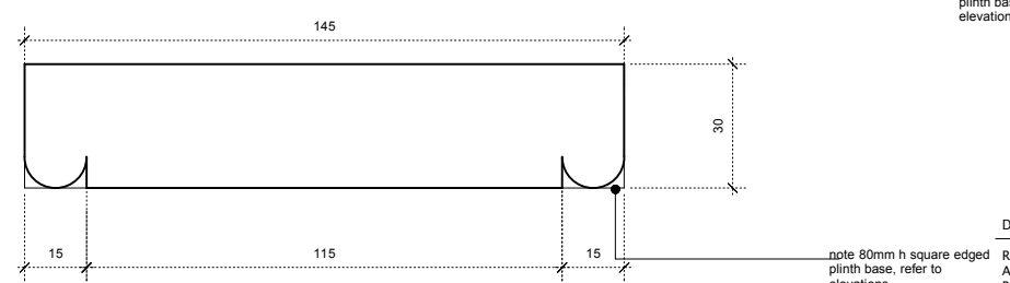
JAMB & HEAD SECTION: FIREPLACE 3 CLOSET ROOM G04 Scale 1:1@A1, 1:2@A3
