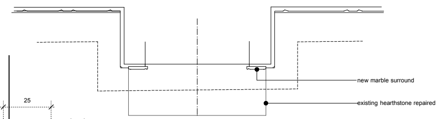
FRONT ROOM (G02) PART PLAN OF FIREPLACE 01 Scale 1:20@A1, 1:40@A3
