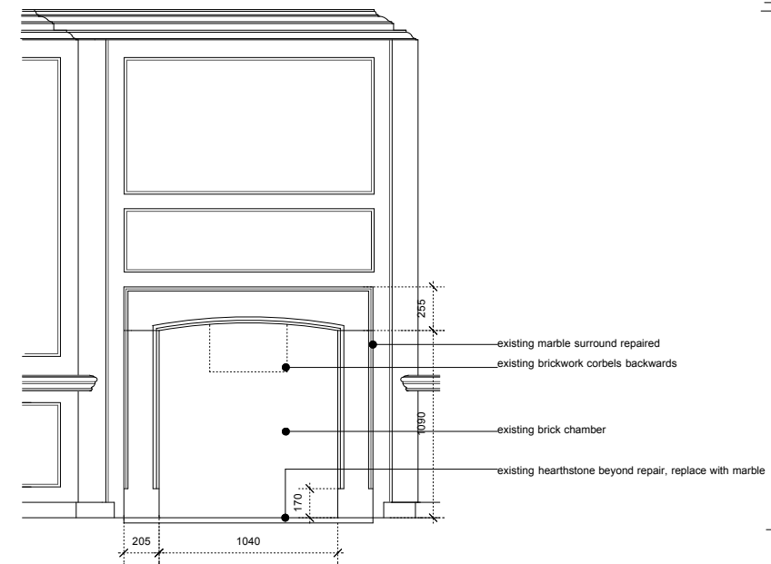
MIDDLE ROOM (G03) FRONT ELEVATION OF FIREPLACE 02 Scale 1:20@A1, 1:40@A3
