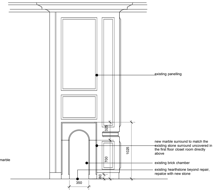
REAR ROOM (G04) FRONT ELEVATION OF FIREPLACE 03 Scale 1:20@A1, 1:40@A3
