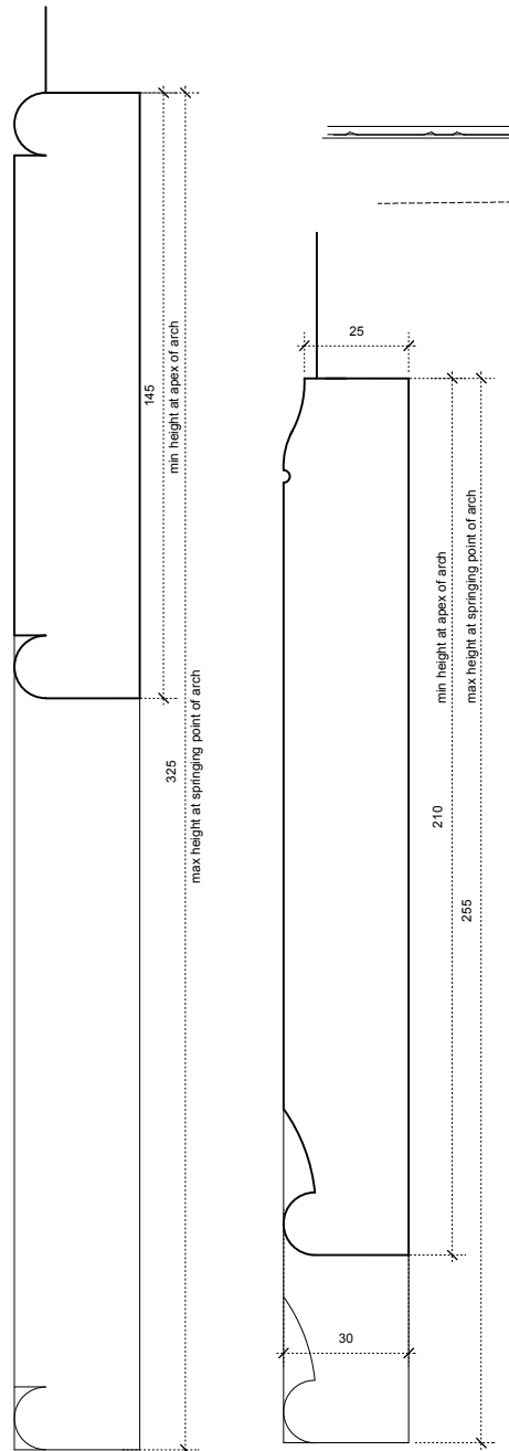
HEAD SECTION: FIREPLACE 3 CLOSET ROOM G04 Scale 1:1@A1, 1:2@A3
