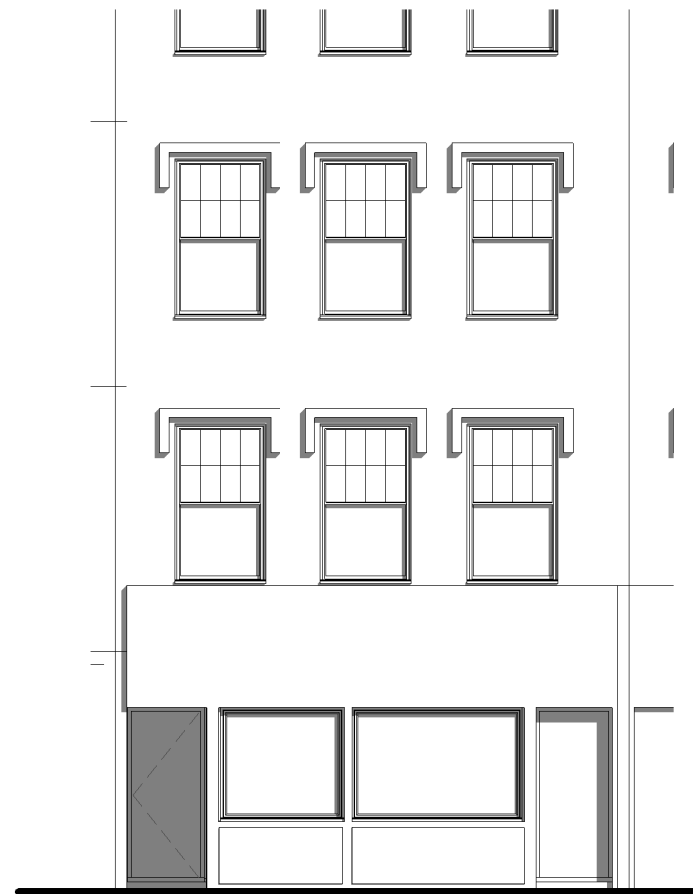
1 Proposed Front Elevation. 1 : 100
