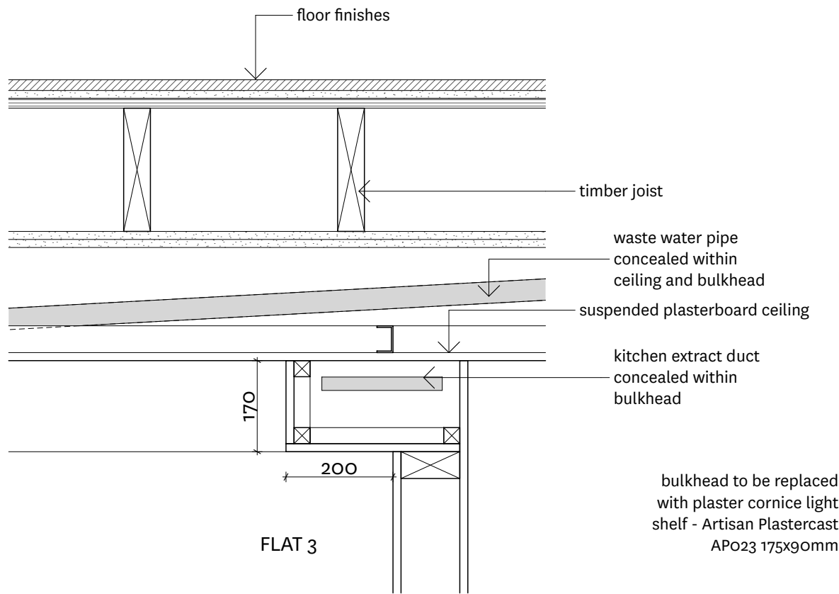
O3. As built
