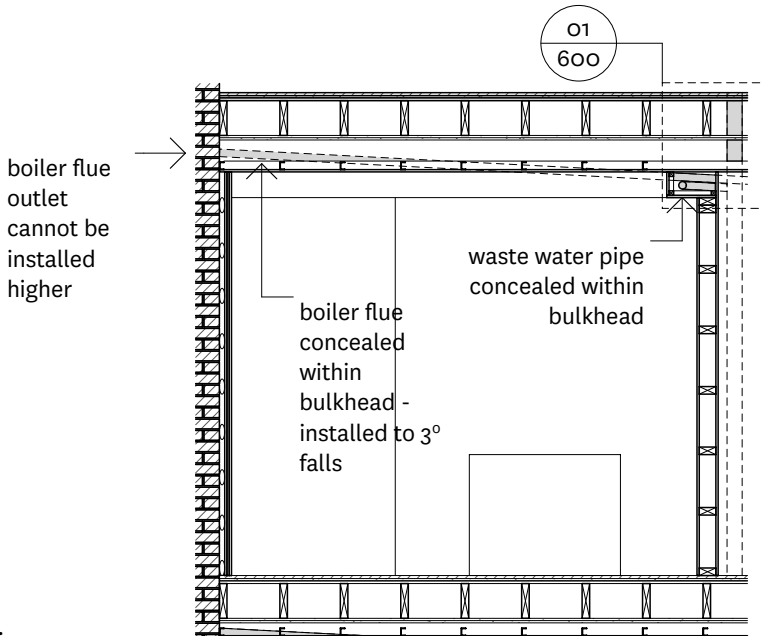
O1. service runs as built 1:50
