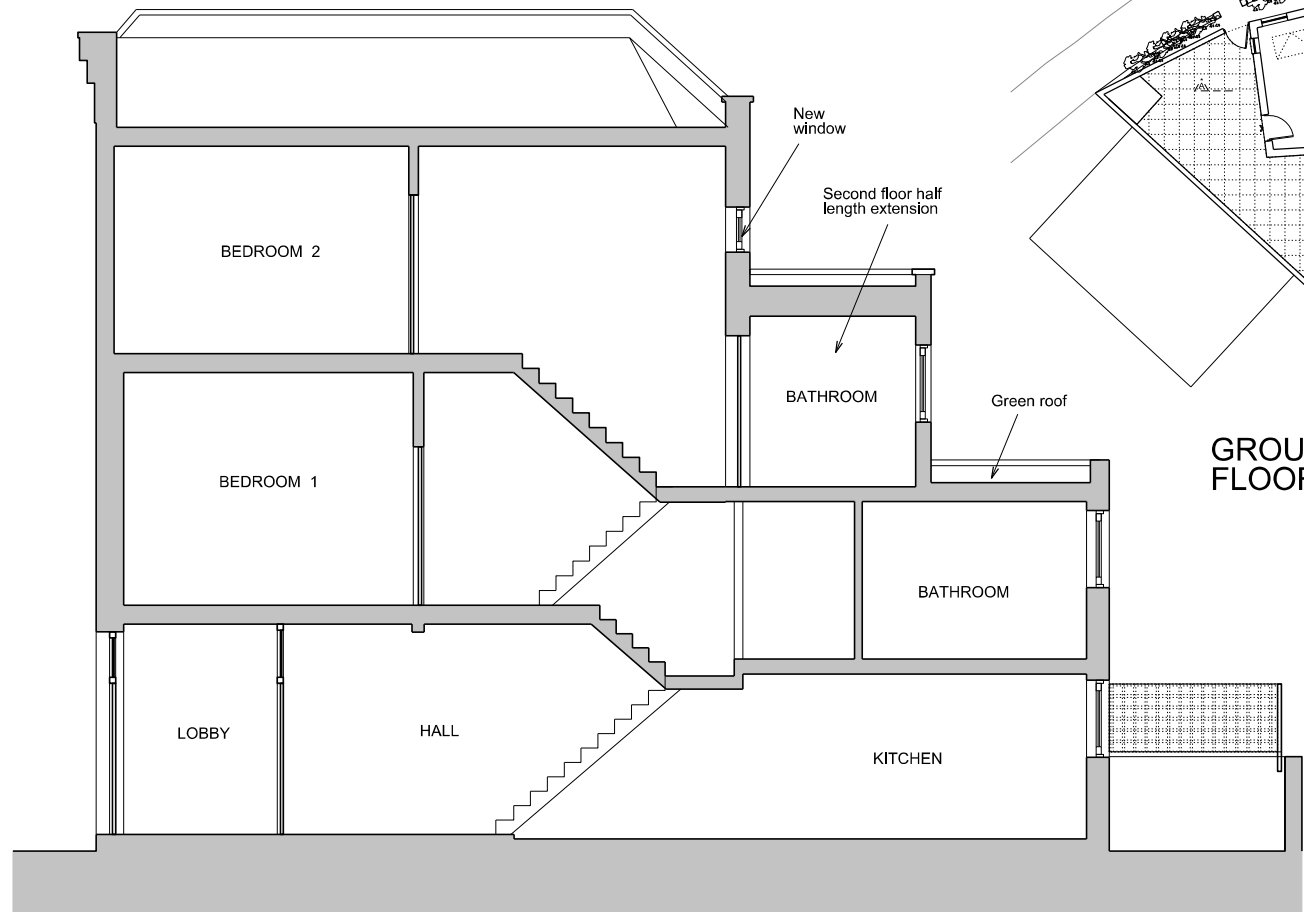
PROPOSED SECTION C-C
