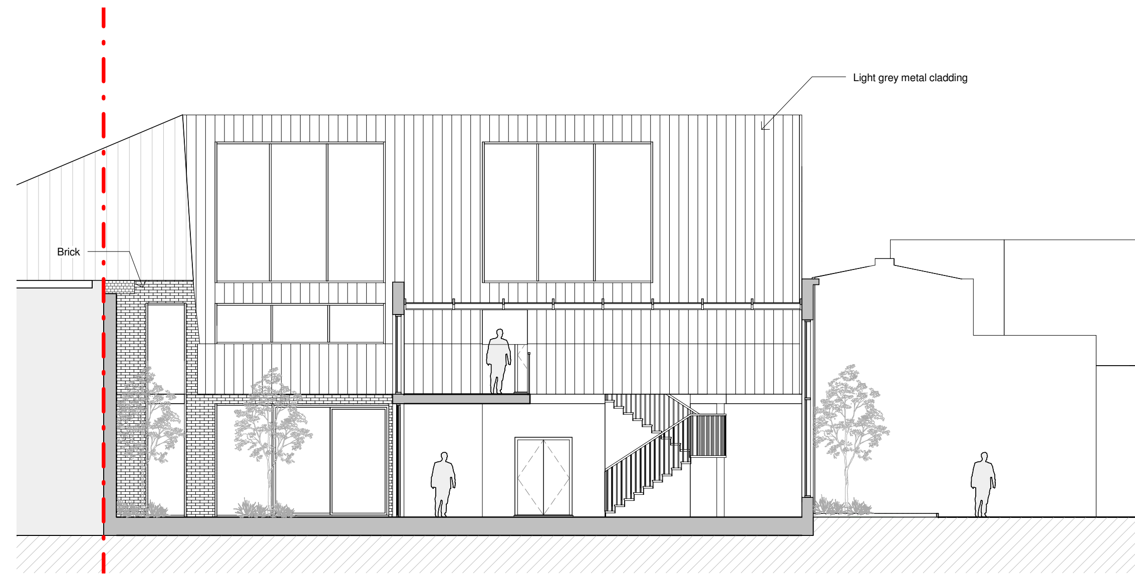
1 Commercial Courtyard 1 : 100
