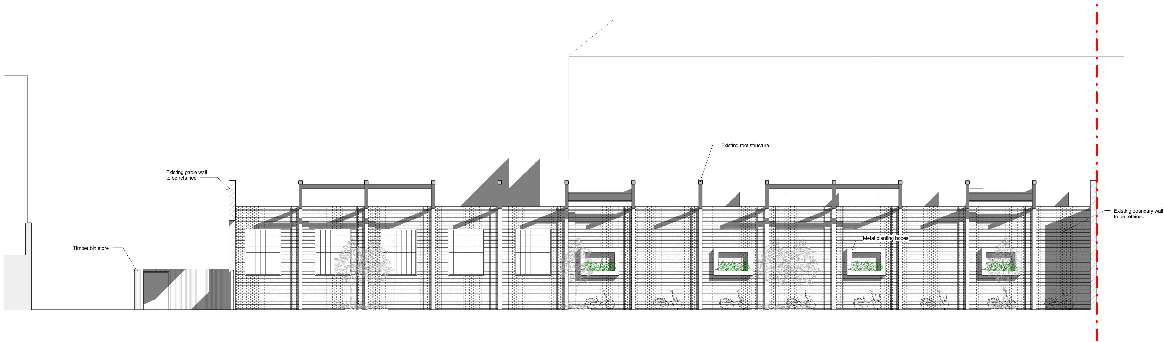
2 Front Boundary Wall 1 : 100
