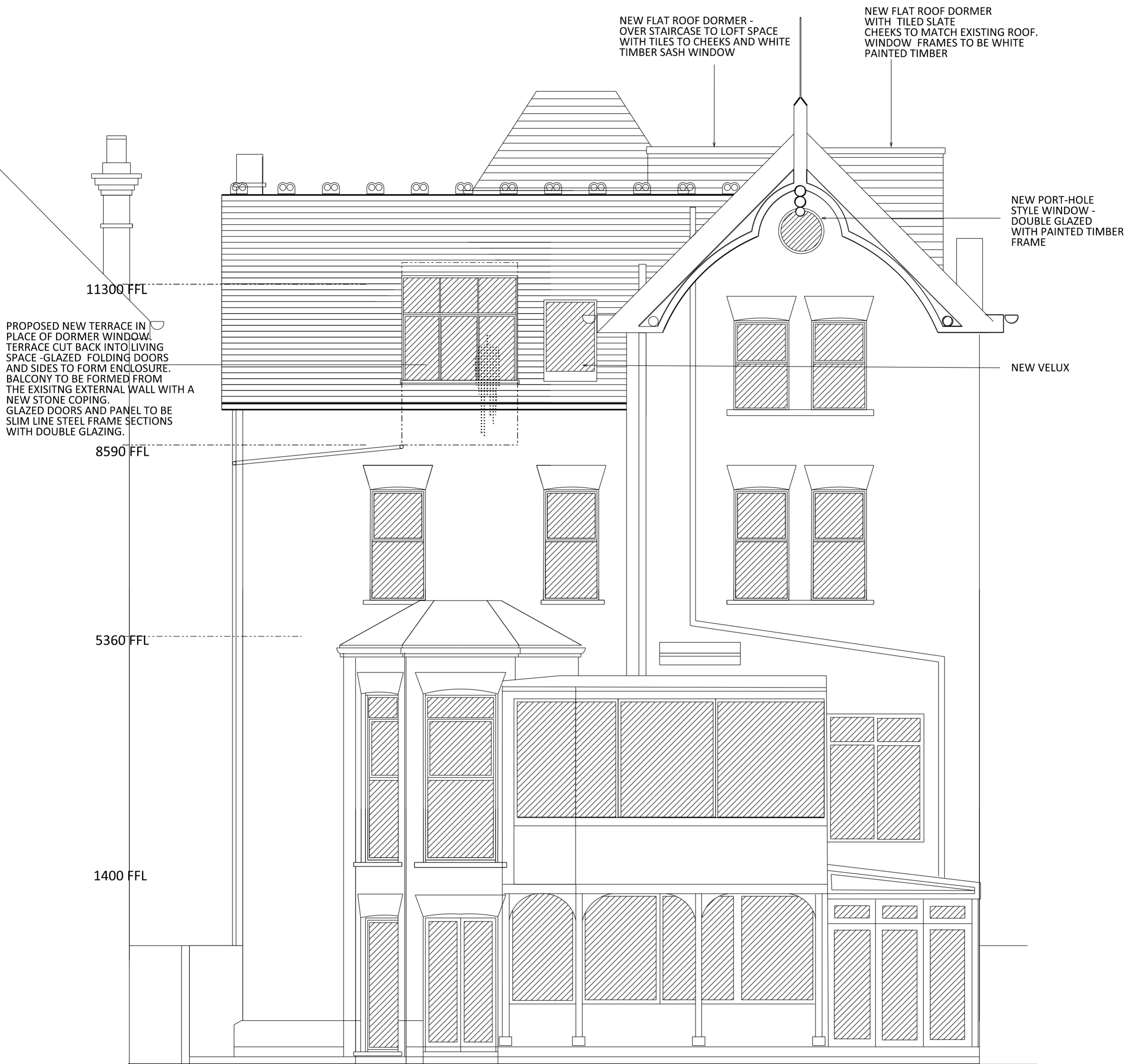
PROPOSED REAR ELEVATION
