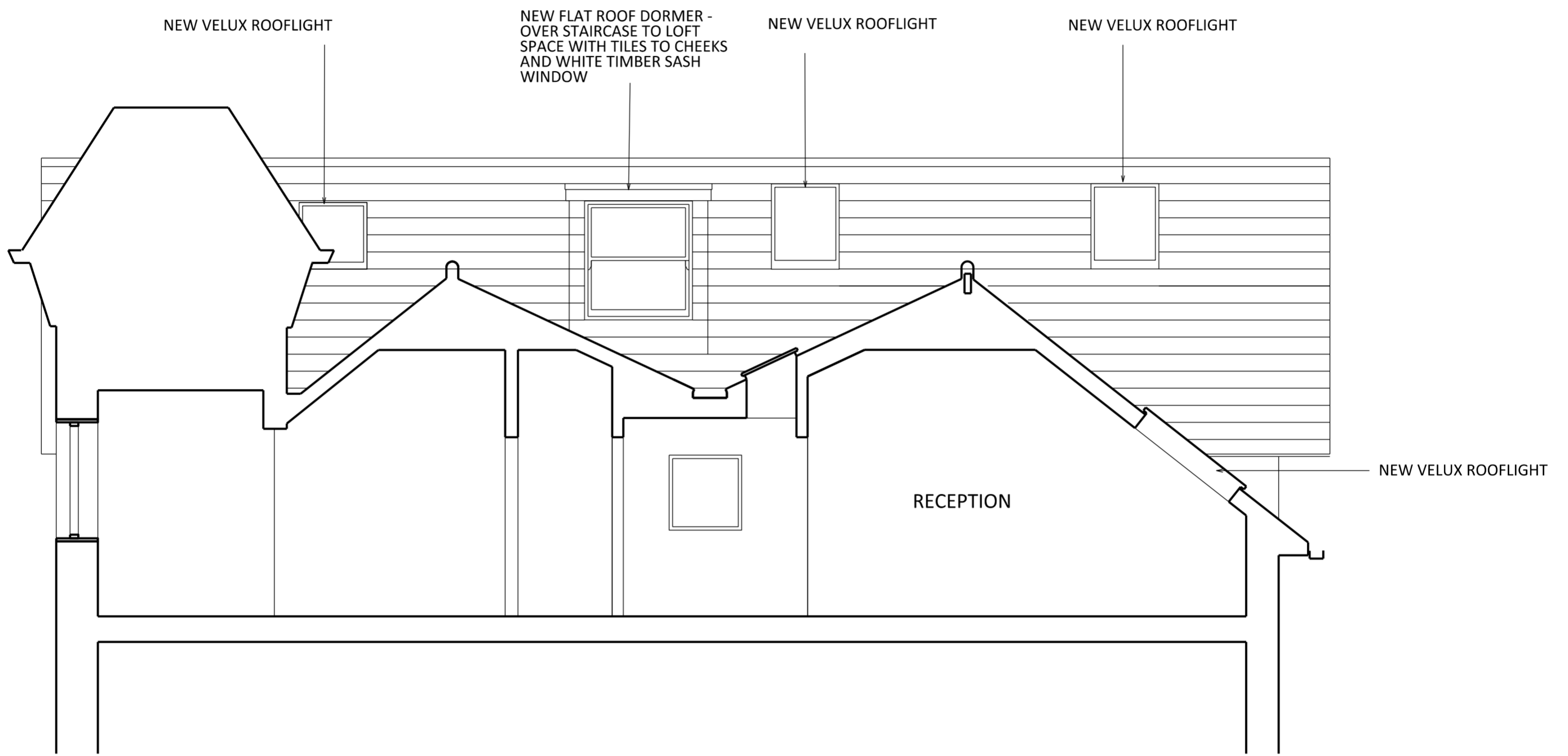
WEST ELEVATION OF LOFT ROOF /SECTION A-A
