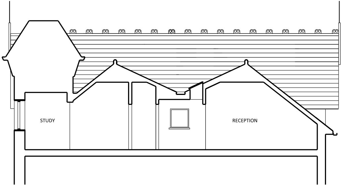
WEST ELEVATION OF LOFT ROOF /SECTION A-A
