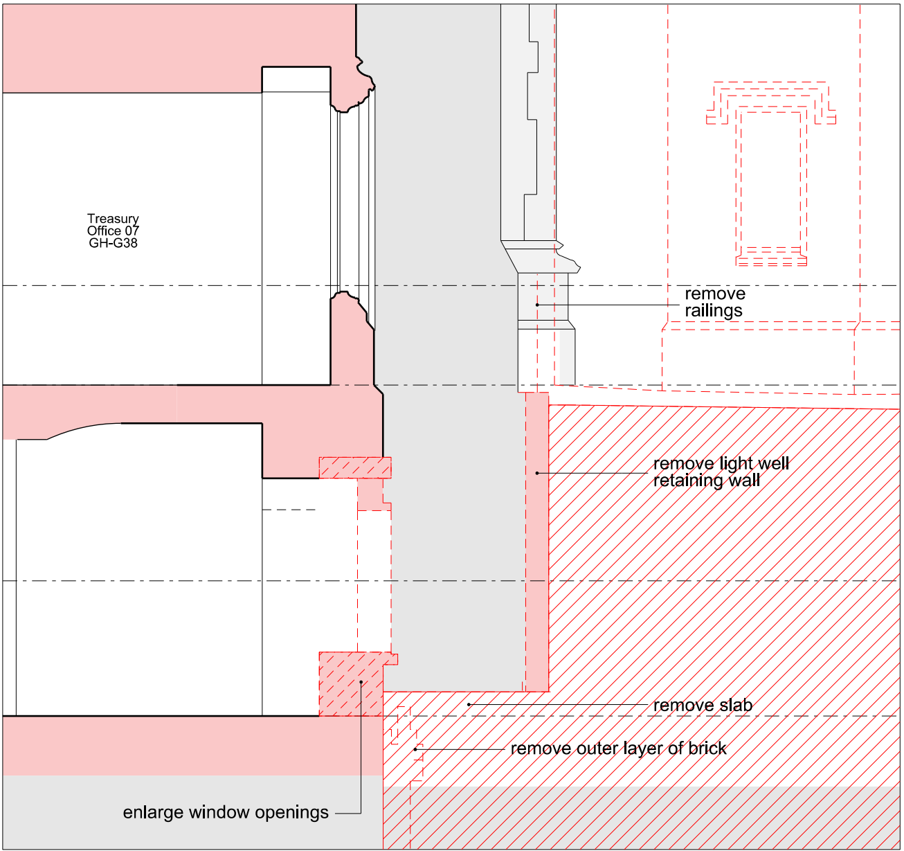
Demolition: Typical Lightwell Rooflight | Short Section
