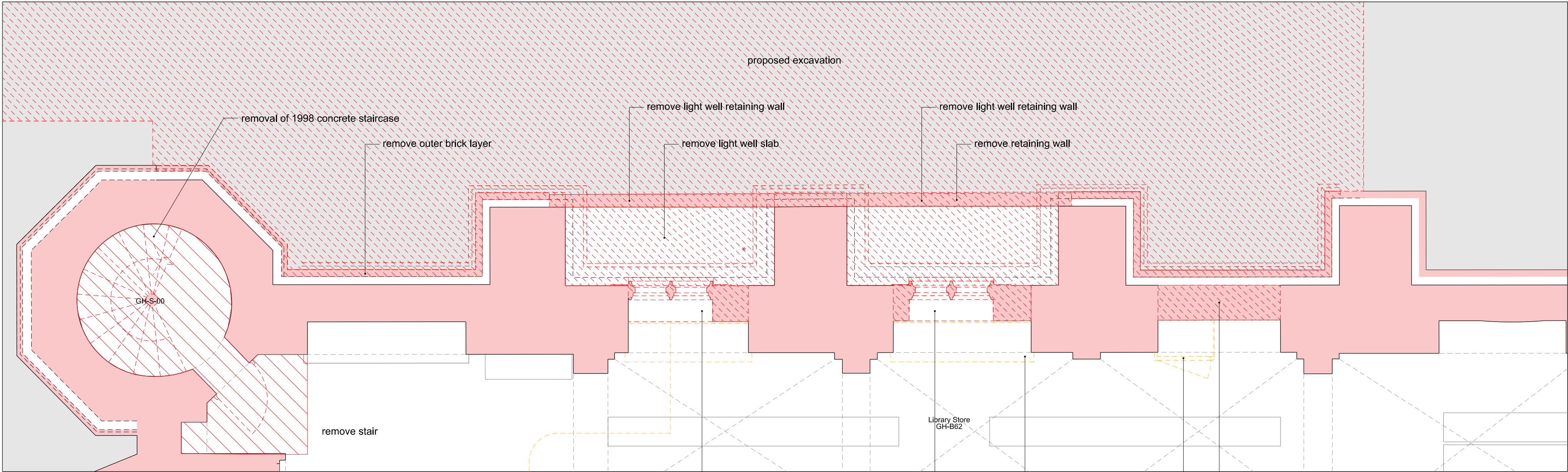
Demolition: Connections to Existing Library Storage | Basement Plan
