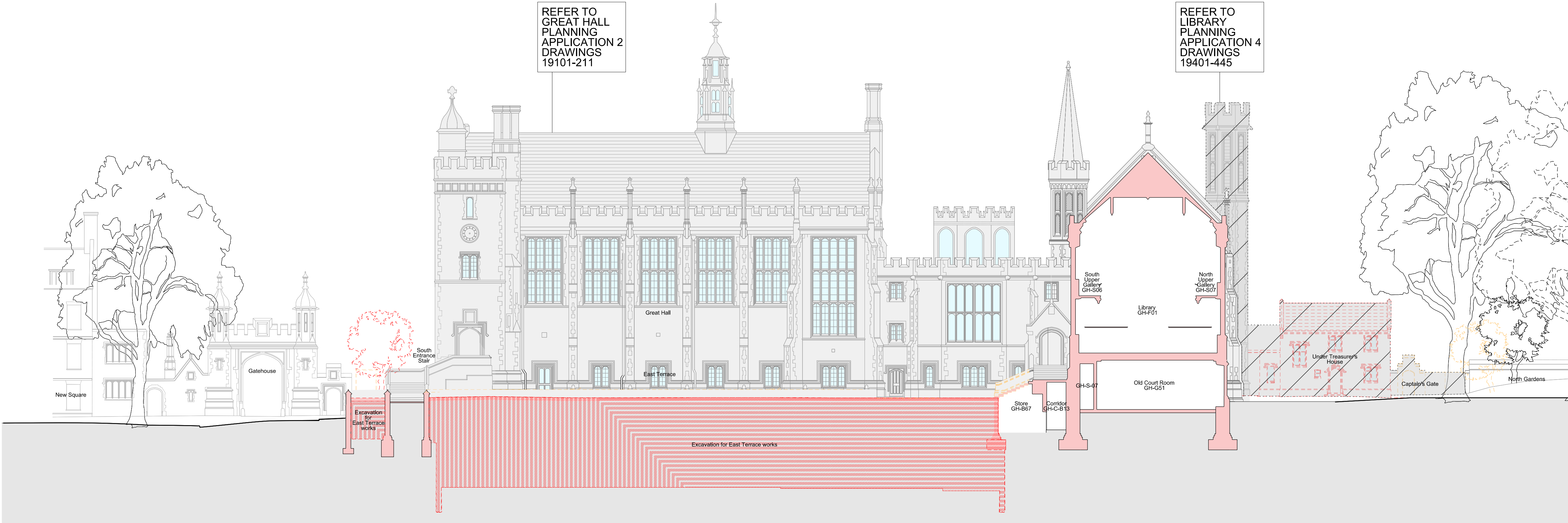
Existing Section J-J with Proposed Demolition
