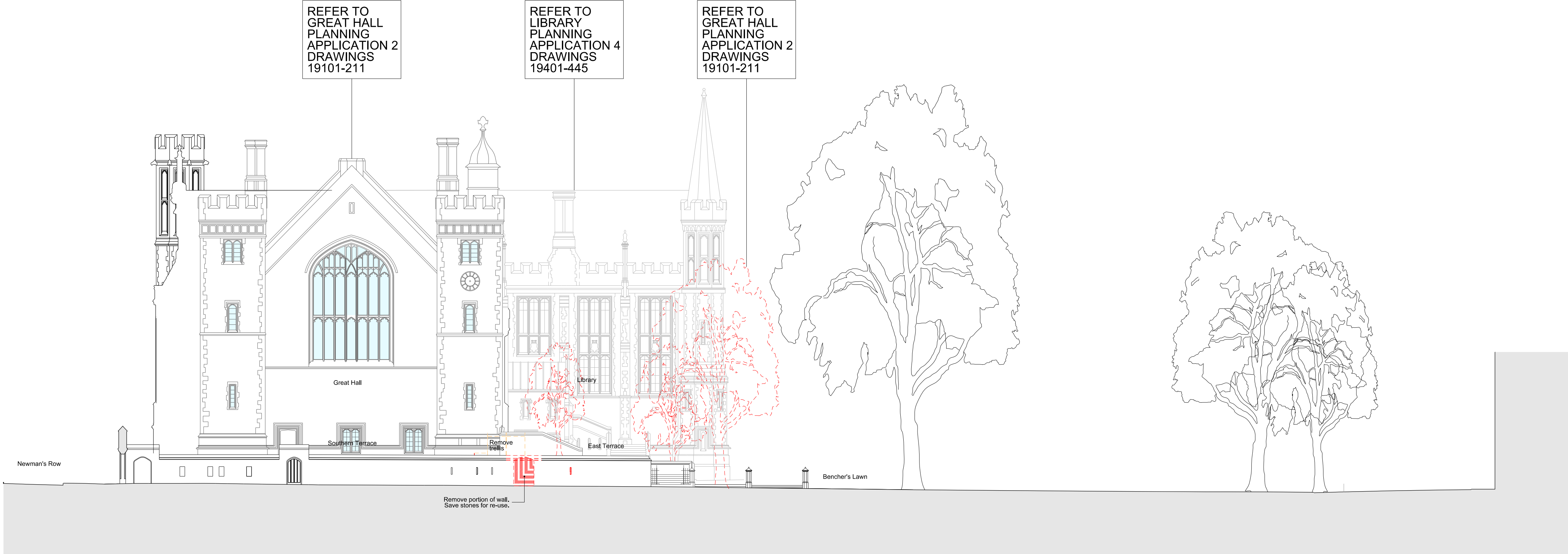
Existing South Elevation with Proposed Demolition
