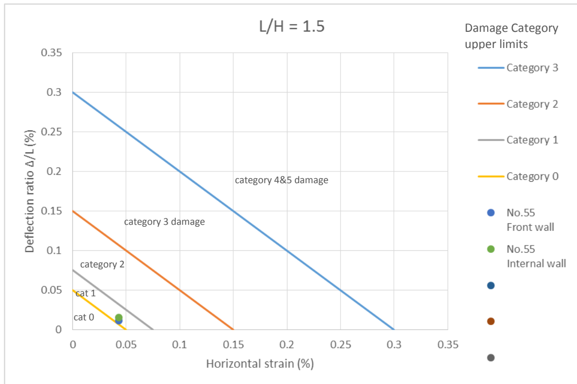
Figure 8: Damage category assessments for front wall of No.55 and any internal transverse walls.
