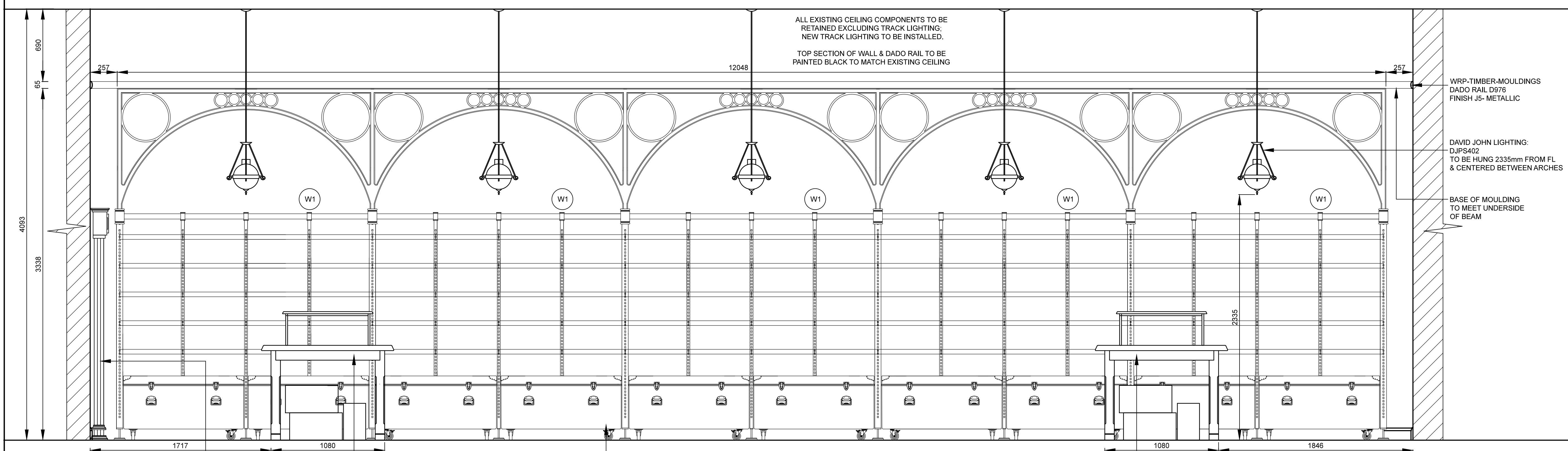
SECTION AA
