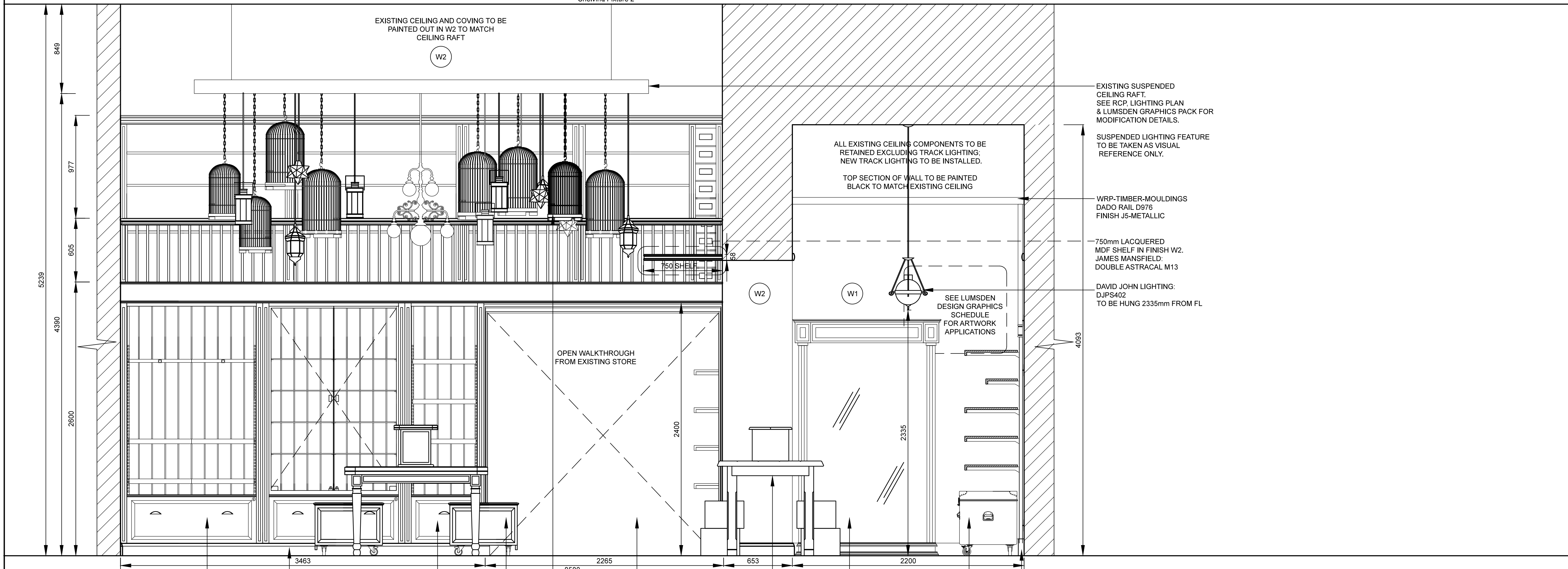
SECTION BB
