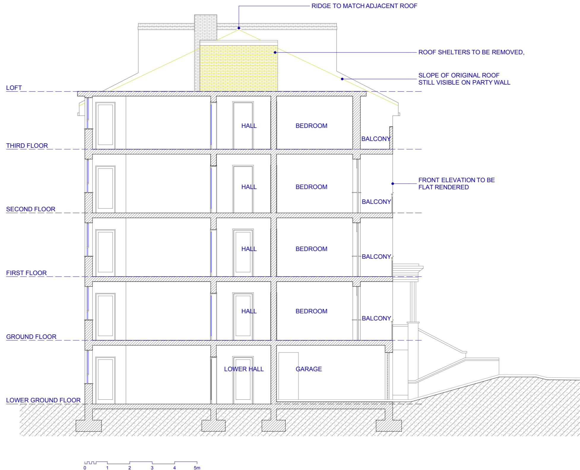
Section C-C as Existing
