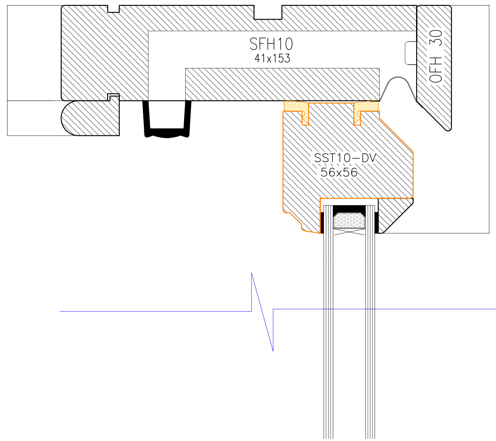
SECTION N Scale 1:1
