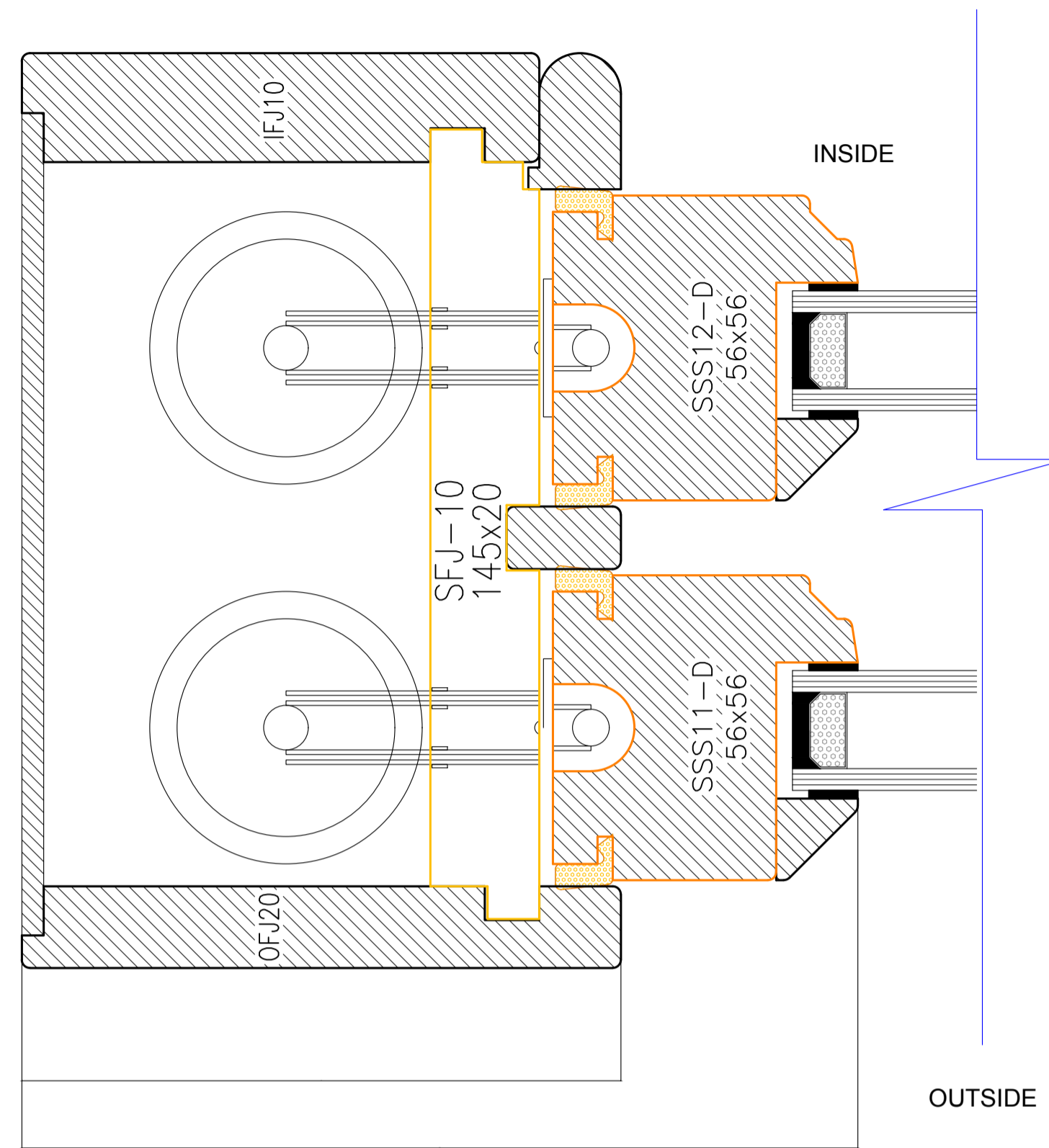
SECTION O Scale 1:1
