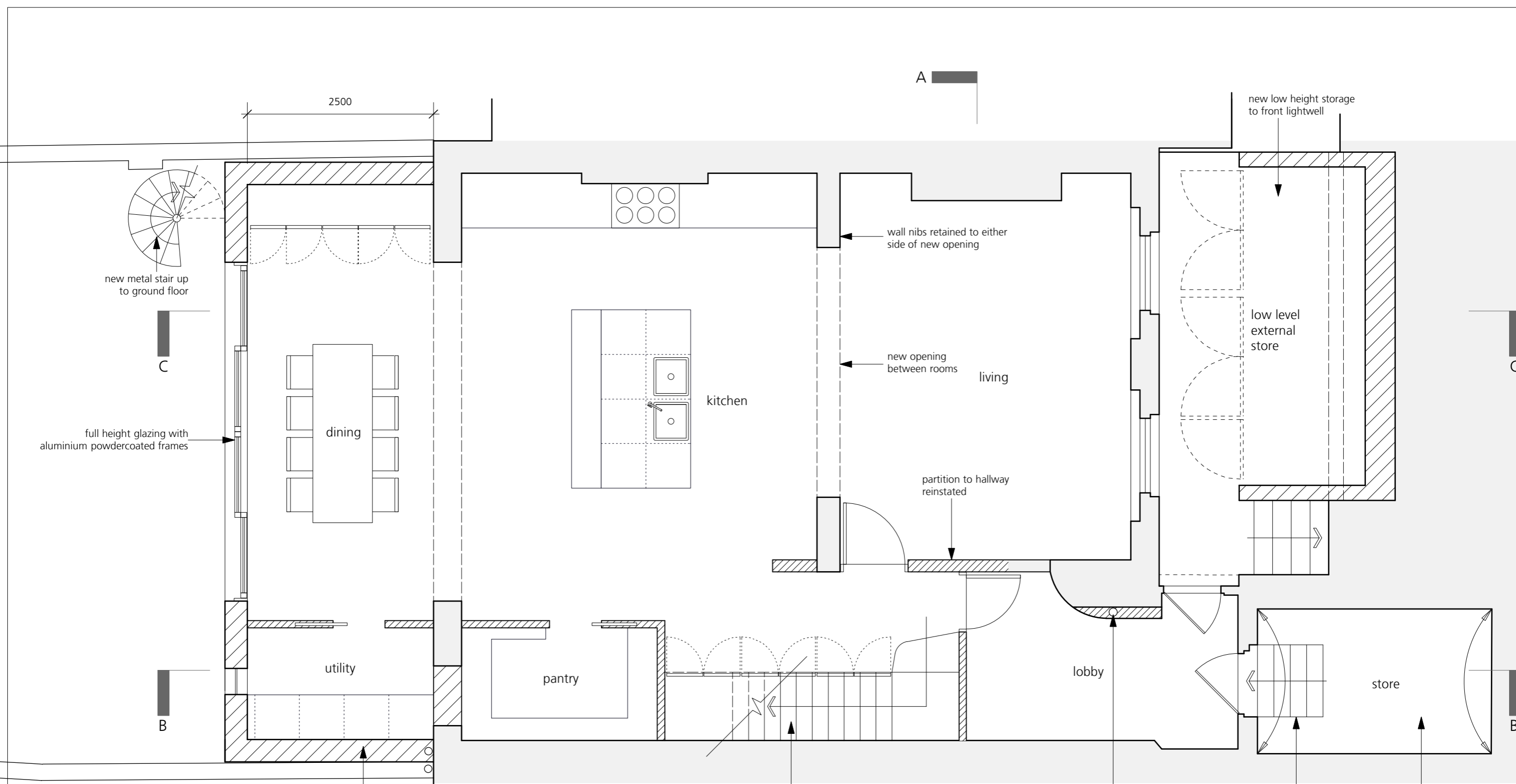
AS PROPOSED Lower Ground Floor Plan
