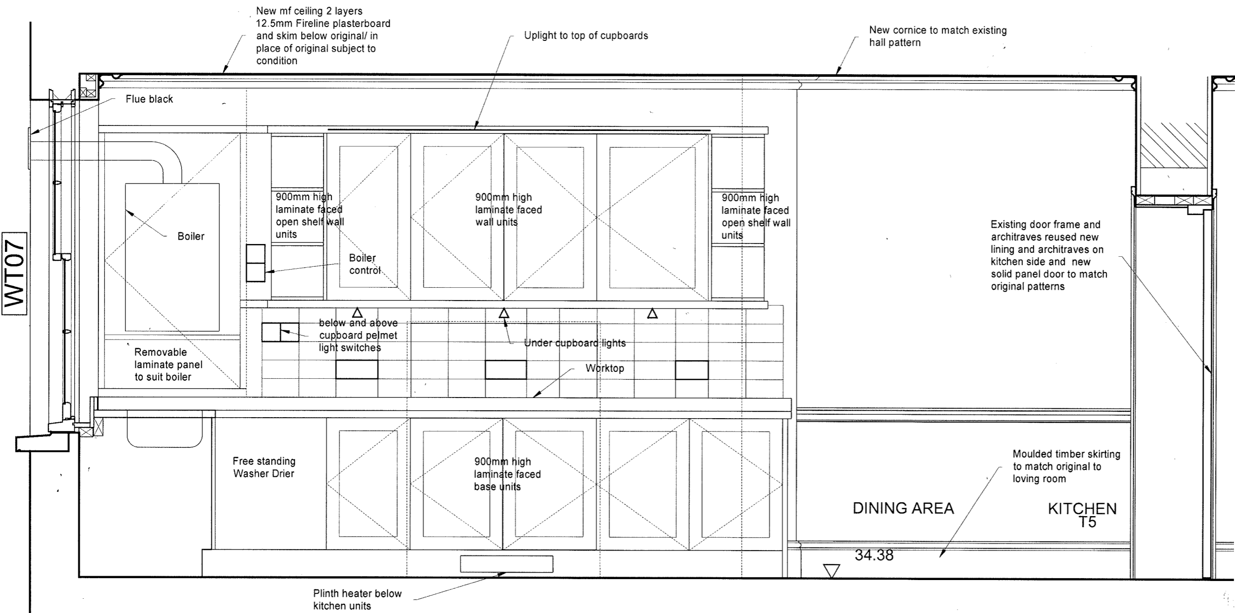
PROPOSED KITCHEN NORTH ELEVATION
