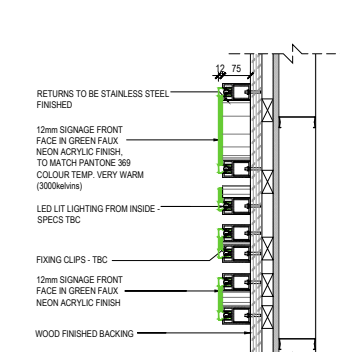
7 BURGER LOGO SECTION SCALE 1:10
