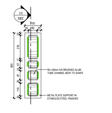
9 BLADE MOUNTED BURGER LOGO SIDE ELEV SCALE 1:10
