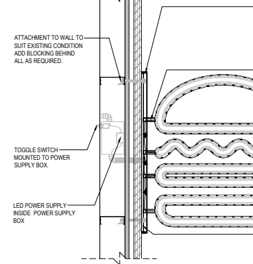
11 BLADE MOUNTED BURGER LOGO SECTION SCALE 1:10
