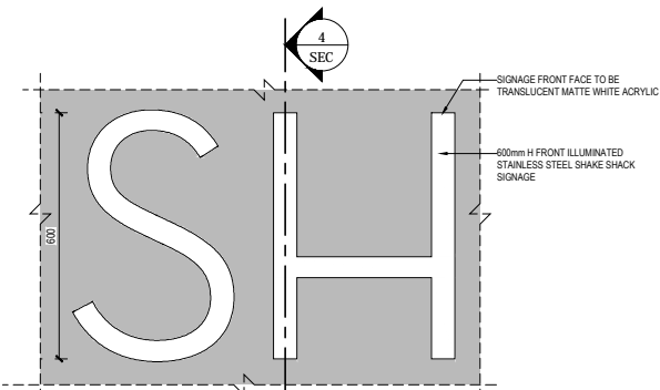
3 SHAKE SHACK SIGNAGE DETAILED ELEVATION SCALE 1:10
