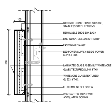
4 SHAKE SHACK SIGNAGE SECTION SCALE 1:10
