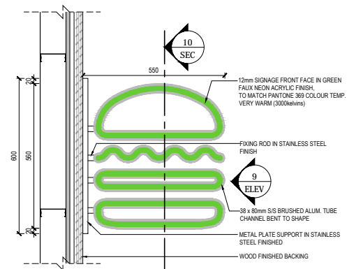
8 BLADE MOUNTED BURGER LOGO ELEV SCALE 1:10
