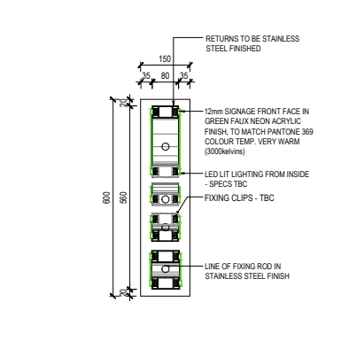
10 BLADE MOUNTED BURGER LOGO SECTION SCALE 1:10
