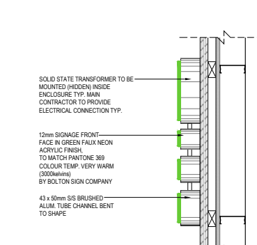
6 BURGER LOGO SIDE ELEVATION SCALE 1:10
