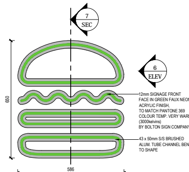
5 BURGER LOGO FRONT ELEVATION SCALE 1:10
