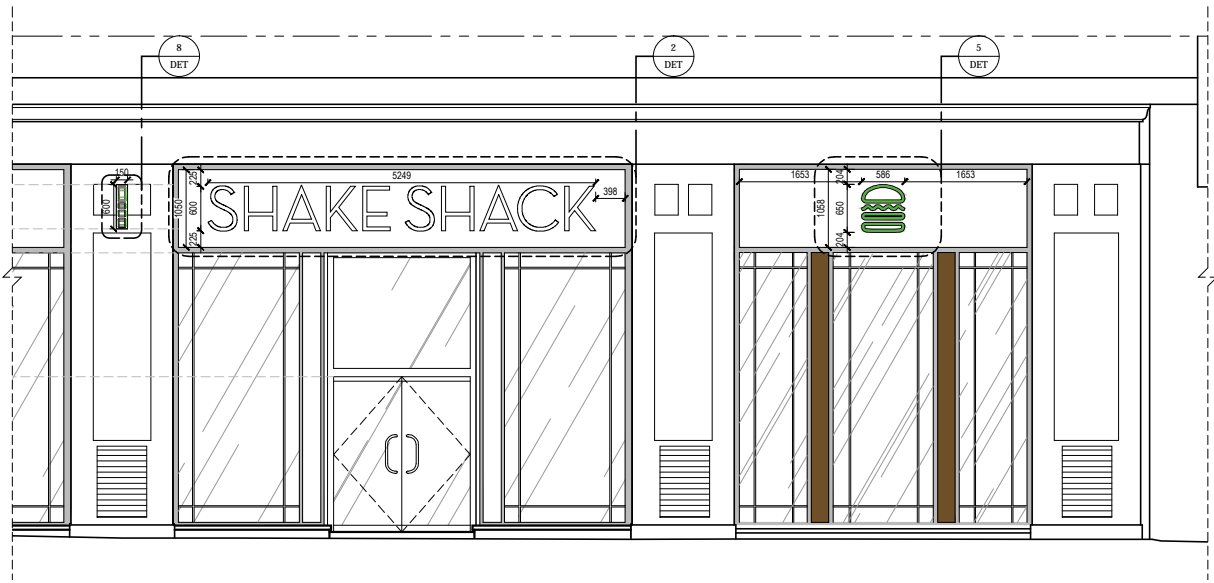
1 STOREFRONT ELEVATION SCALE 1:50
