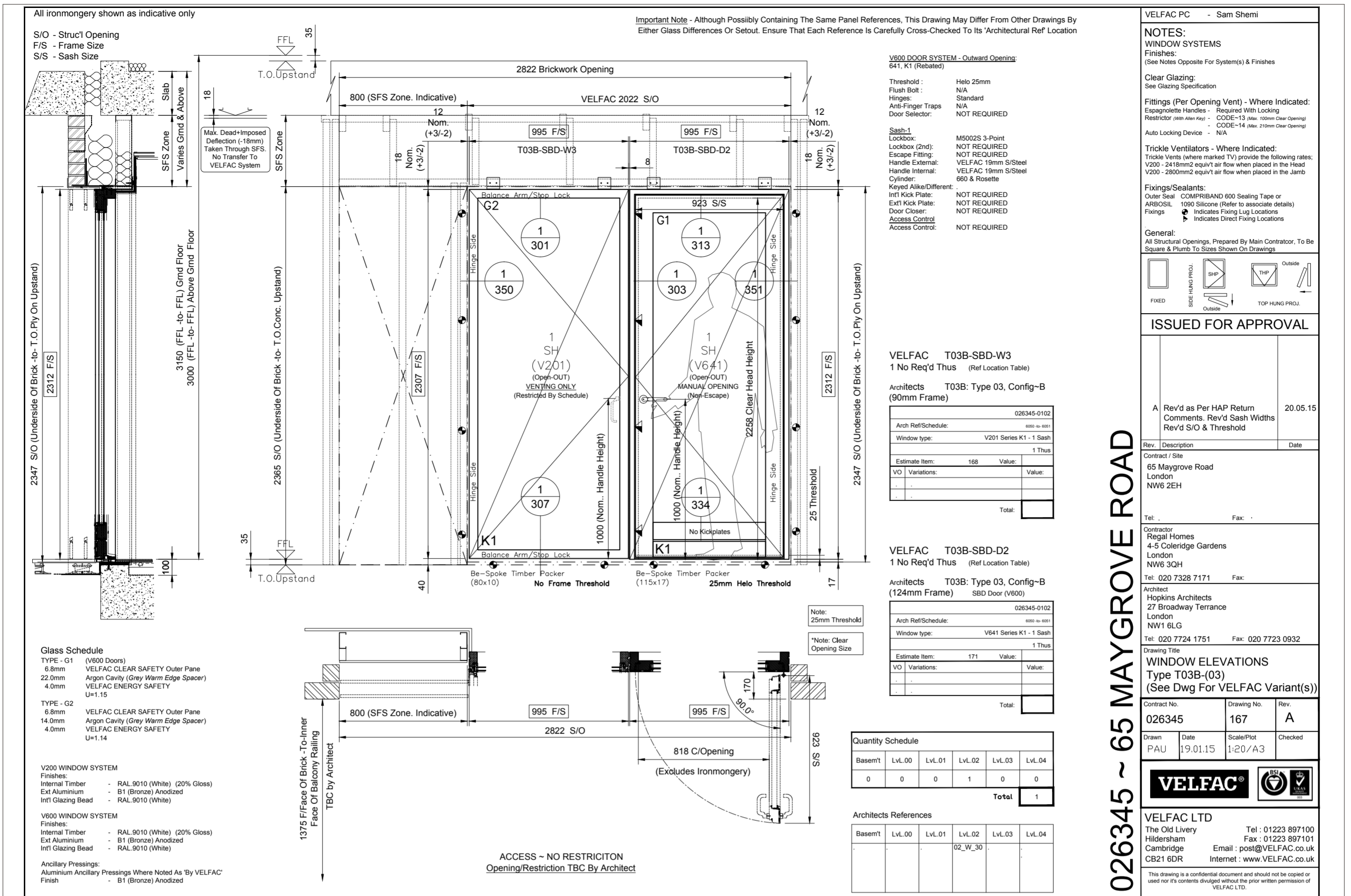
Velfac fabrication drawing
