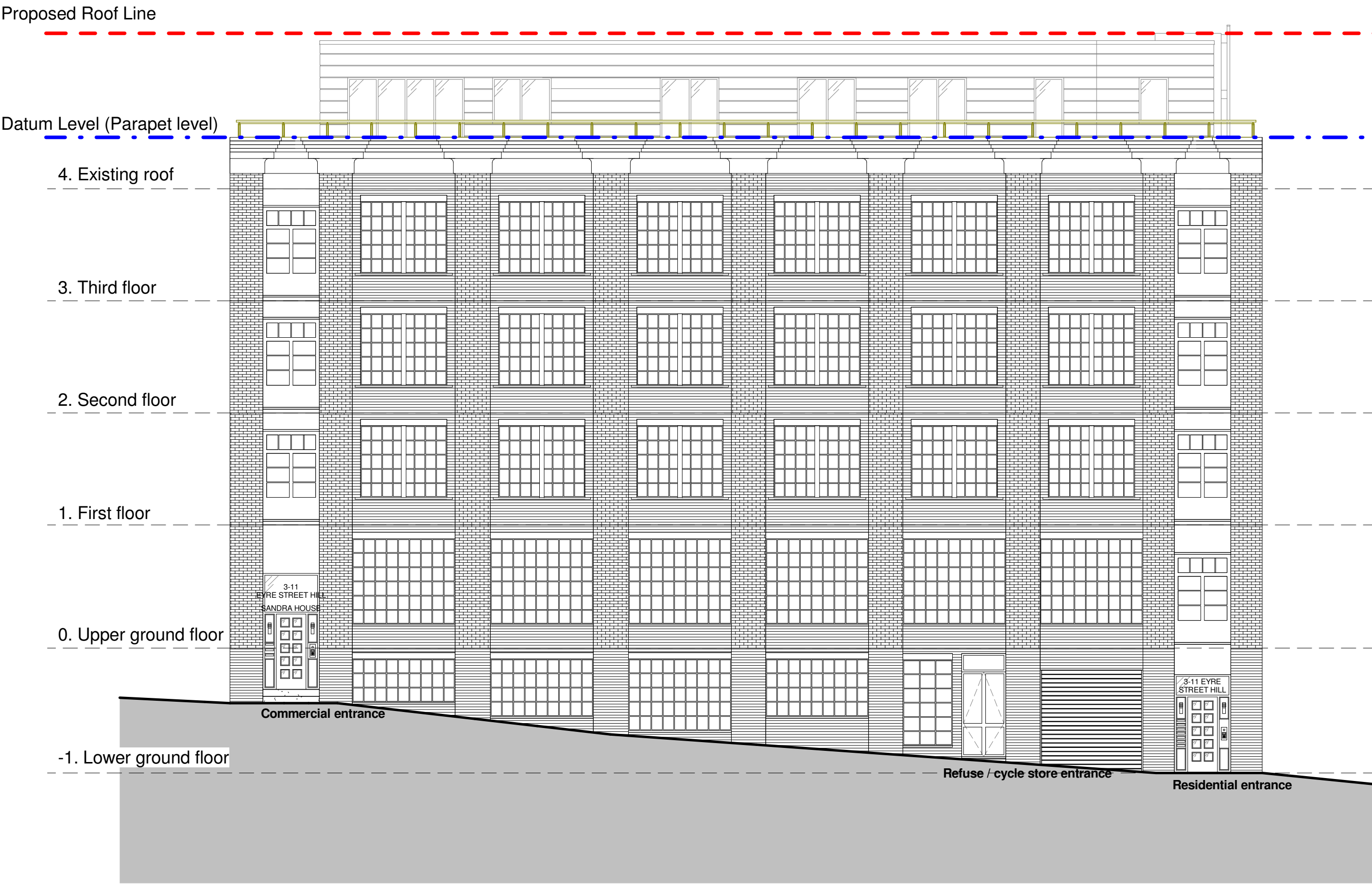
Proposed Elevation
