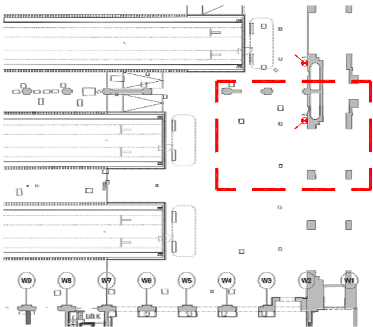
SITE LAYOUT PLAN Scale 1/400
