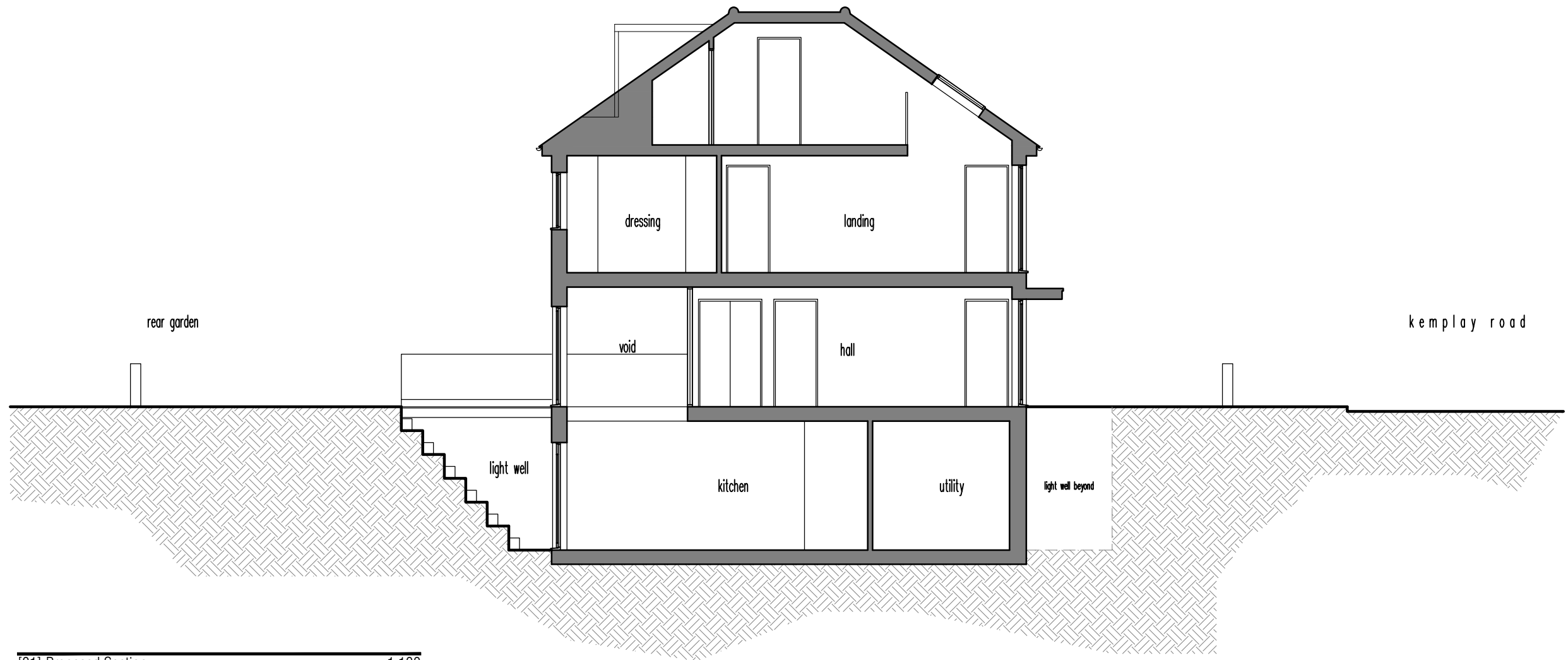
[01] Proposed Section 1:100
