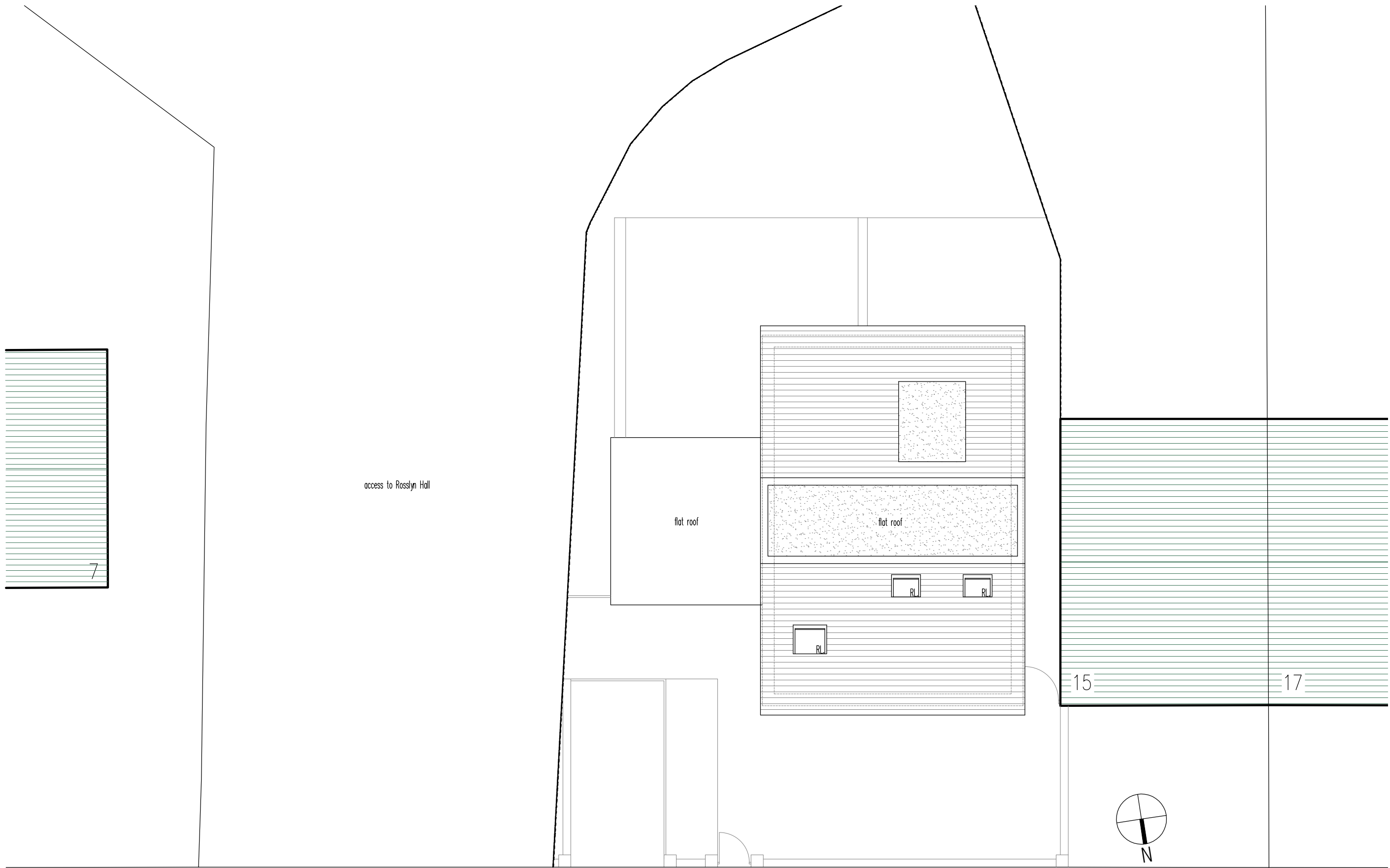
[01] PROPOSED ROOF PLAN 1:100
