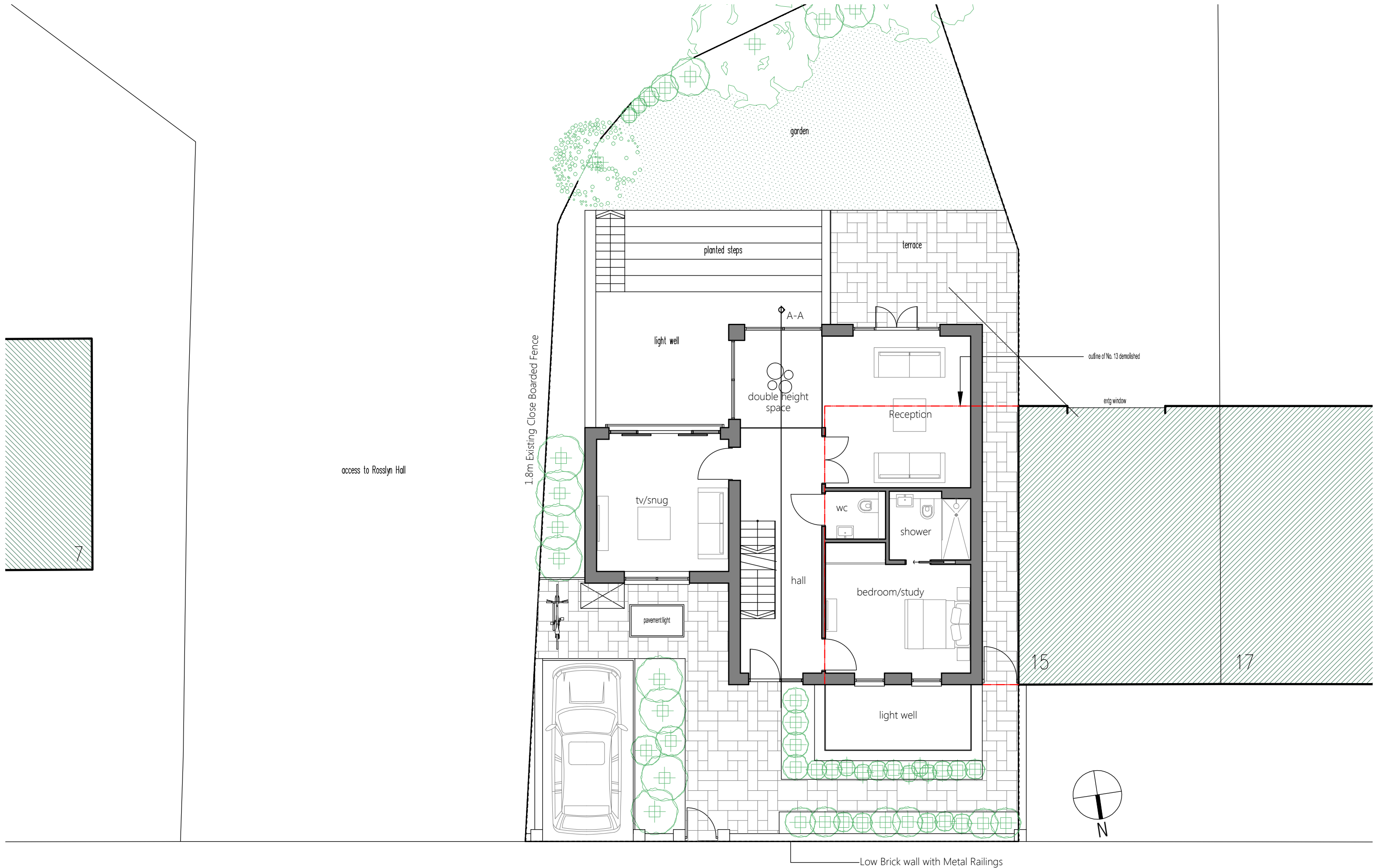
[01] PROPOSED GROUND FLOOR PLAN 1:100
