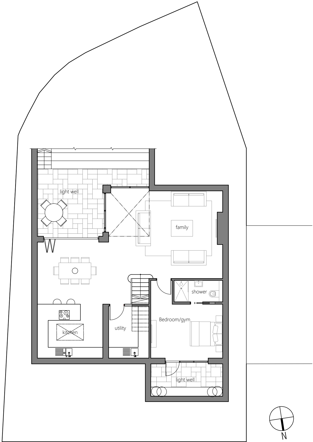
[01] PROPOSED BASEMENT PLAN 1:100
