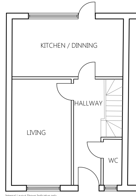
[02] EXISTING GROUND FLOOR PLAN 1:100
