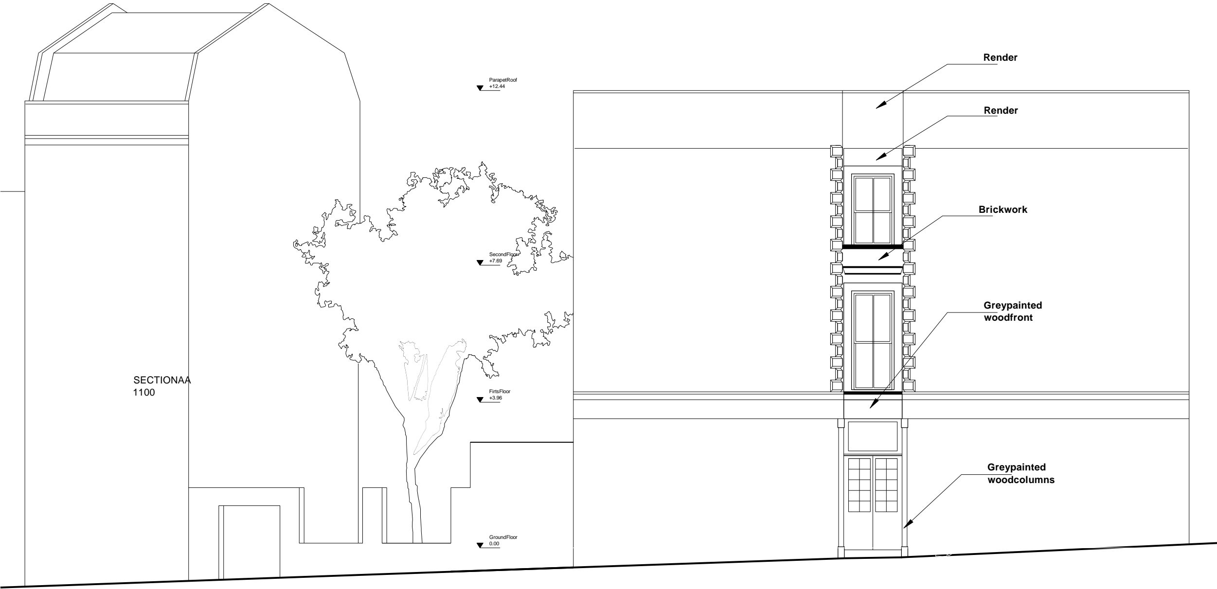
ELEVATION_BRECKNOCKROADTORRIANOAVENUE 1100
