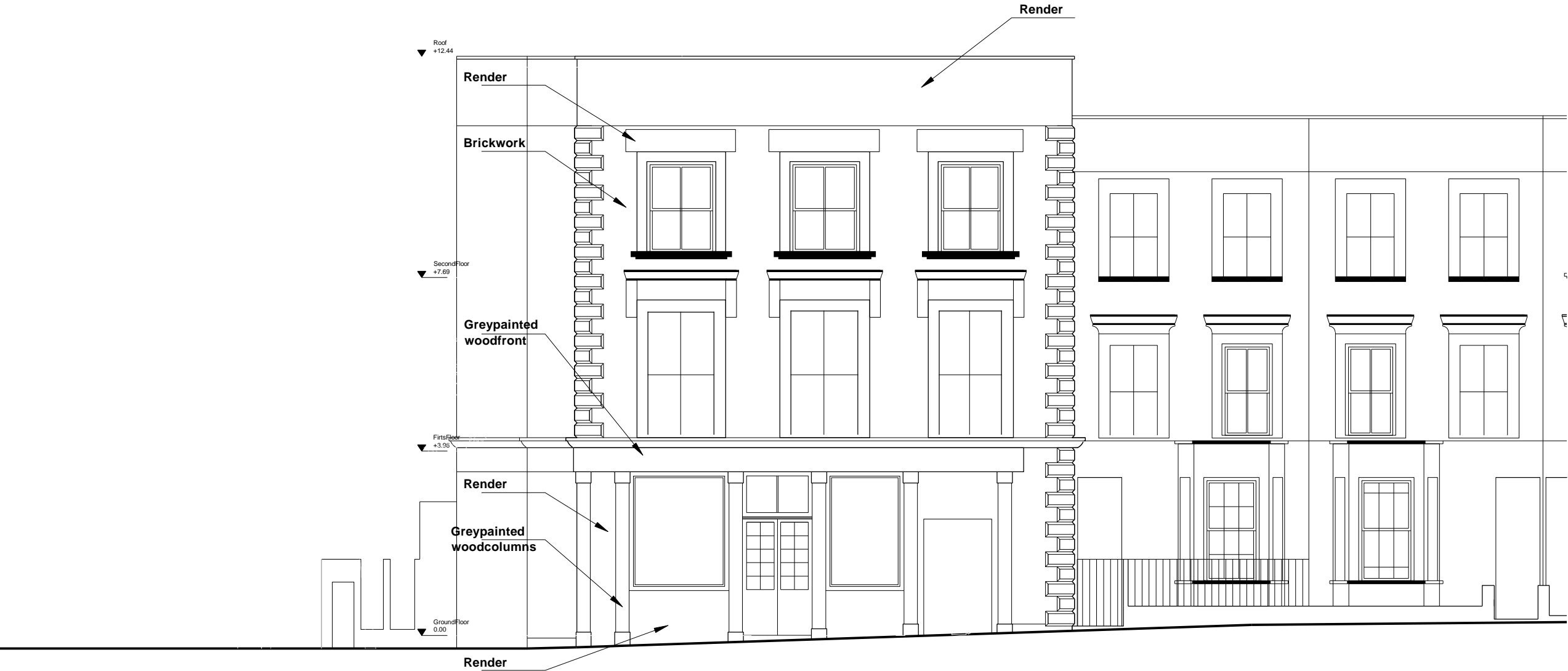
ELEVATION_BRECKNOCKROAD 1100
