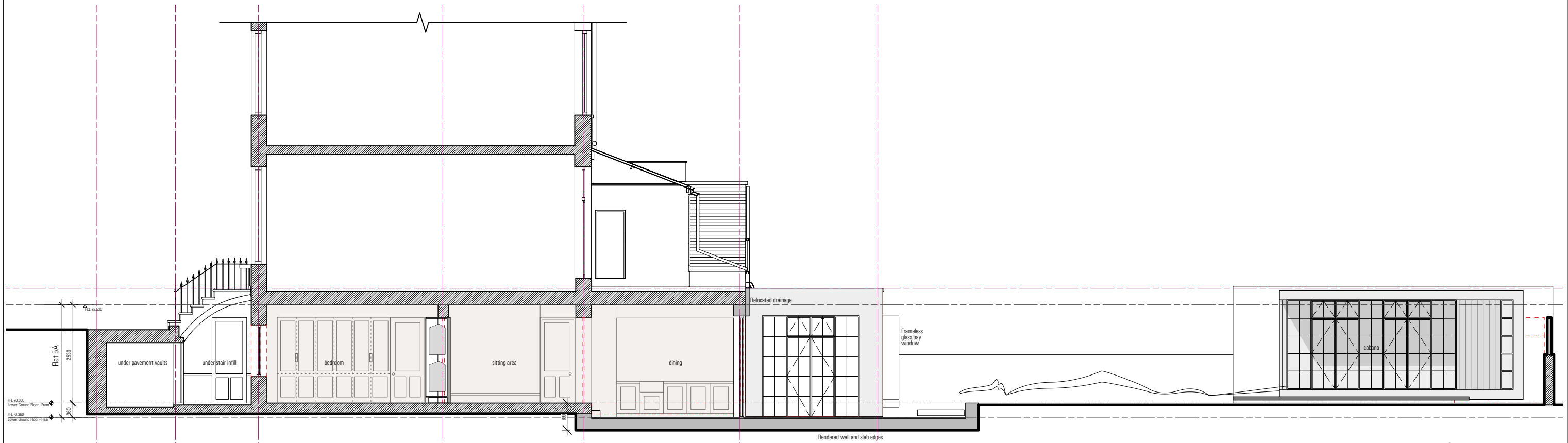
01 Proposed Section A-A Scale 1:100@A3
