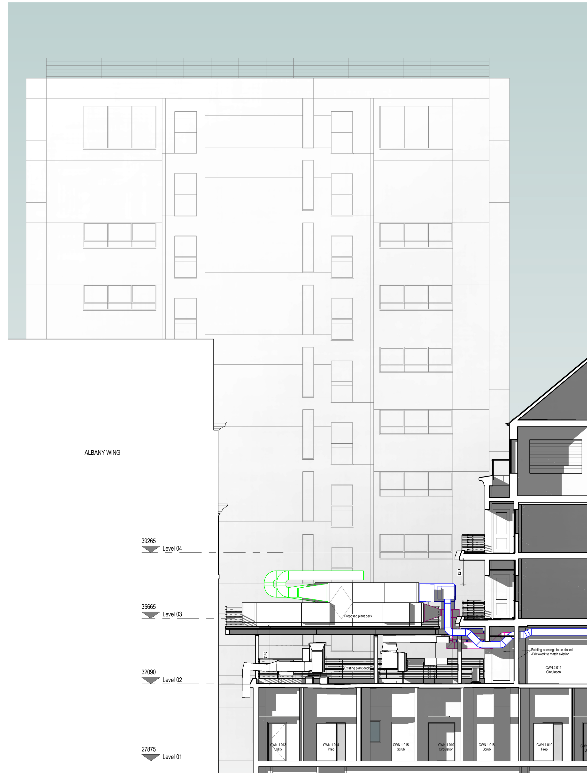
1 Proposed North Section 1 : 100
