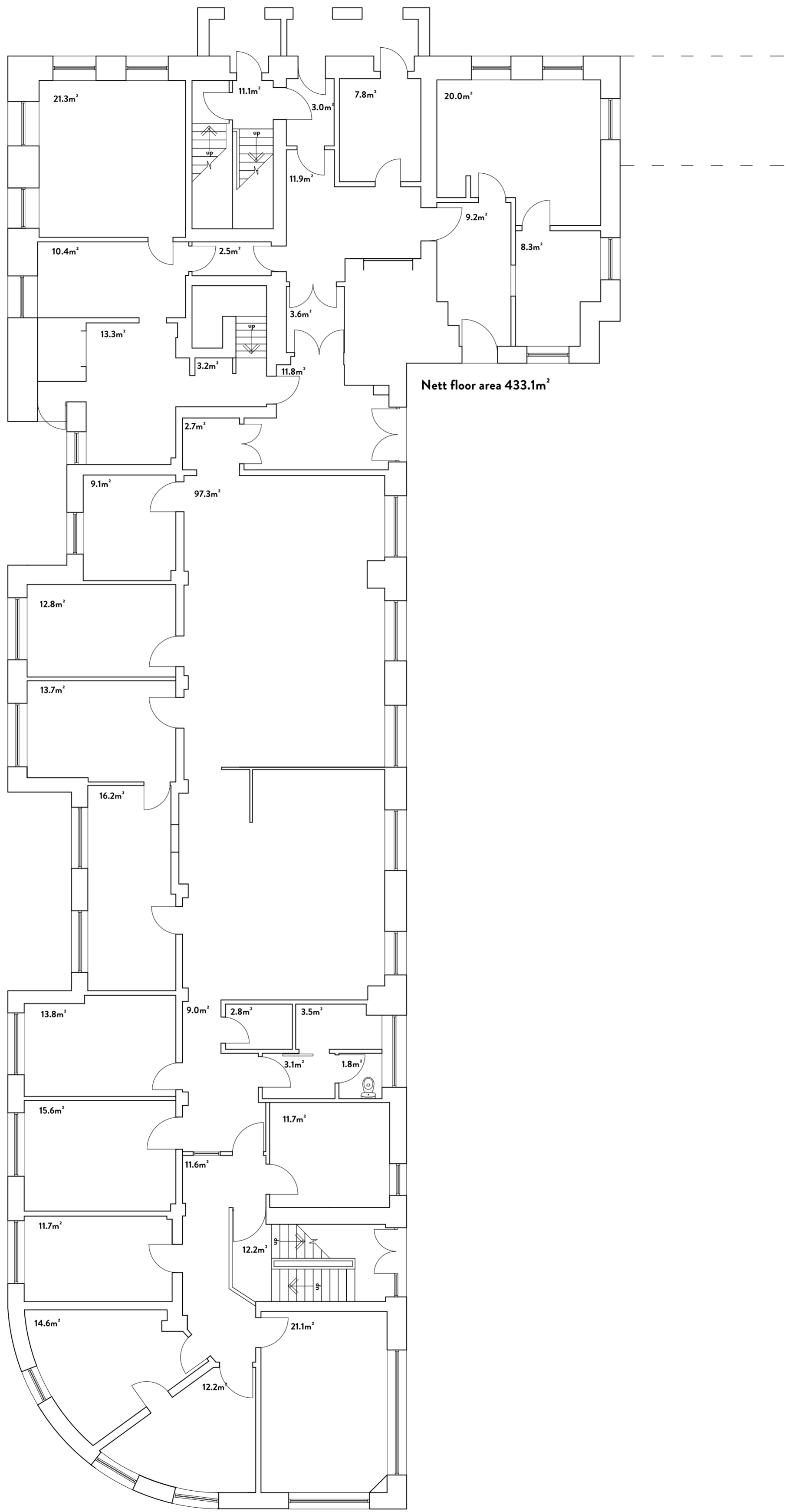
Existing Ground Floor Plan National Temperance Hospital Insull Wing Hampstead Road London
