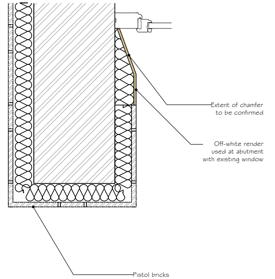
DO5_C - BUTTRESS DETAIL
