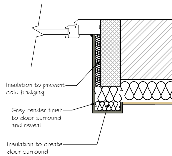
DO5_B - BALCONY DOOR
