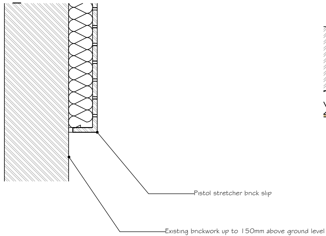
DO5_D - BRICK SLIPS BASE
