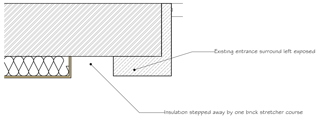
DOI_G - ENTRANCE DETAIL
