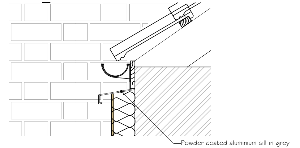
DOI_C - BUTTRESS EAVES
