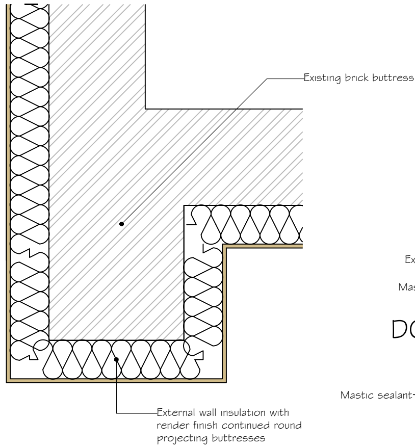
DOI_A BUTTRESS PLAN
