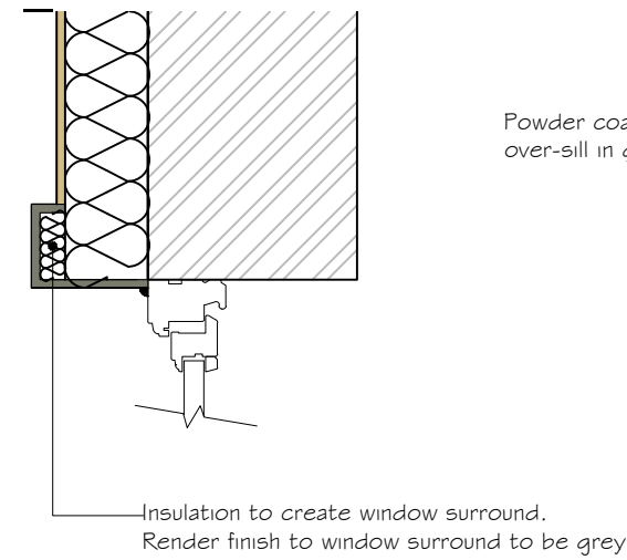
DOI_E - WINDOW HEAD
