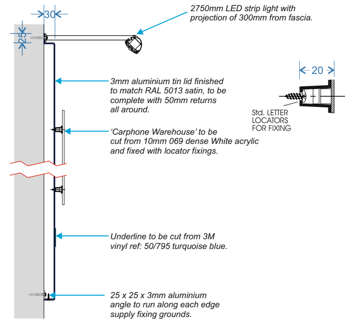
Signage section Scale 1:10
