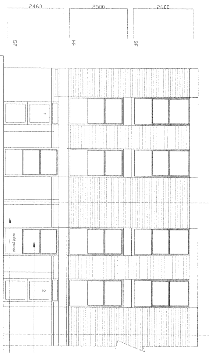
PROPOSED PLAN ELEVATION
