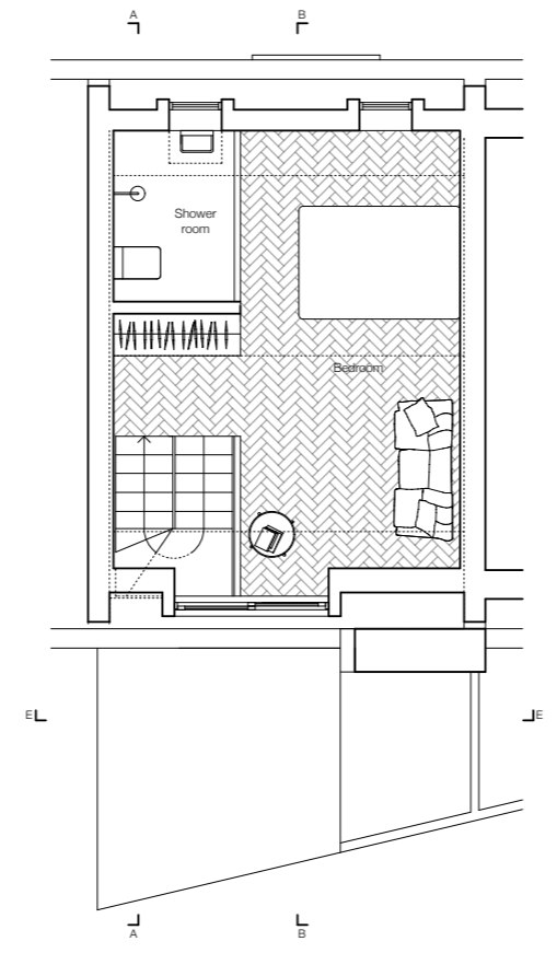
Proposed Third Floor Plan
