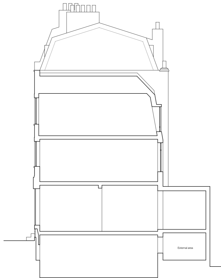
Existing Section B
