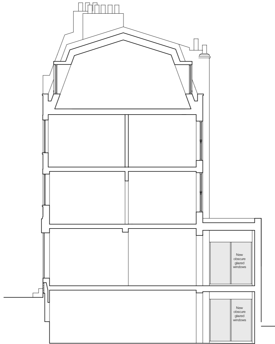
Proposed Section B
