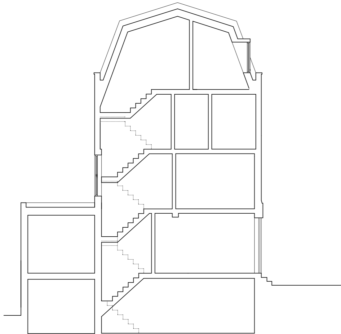
Proposed Section A
