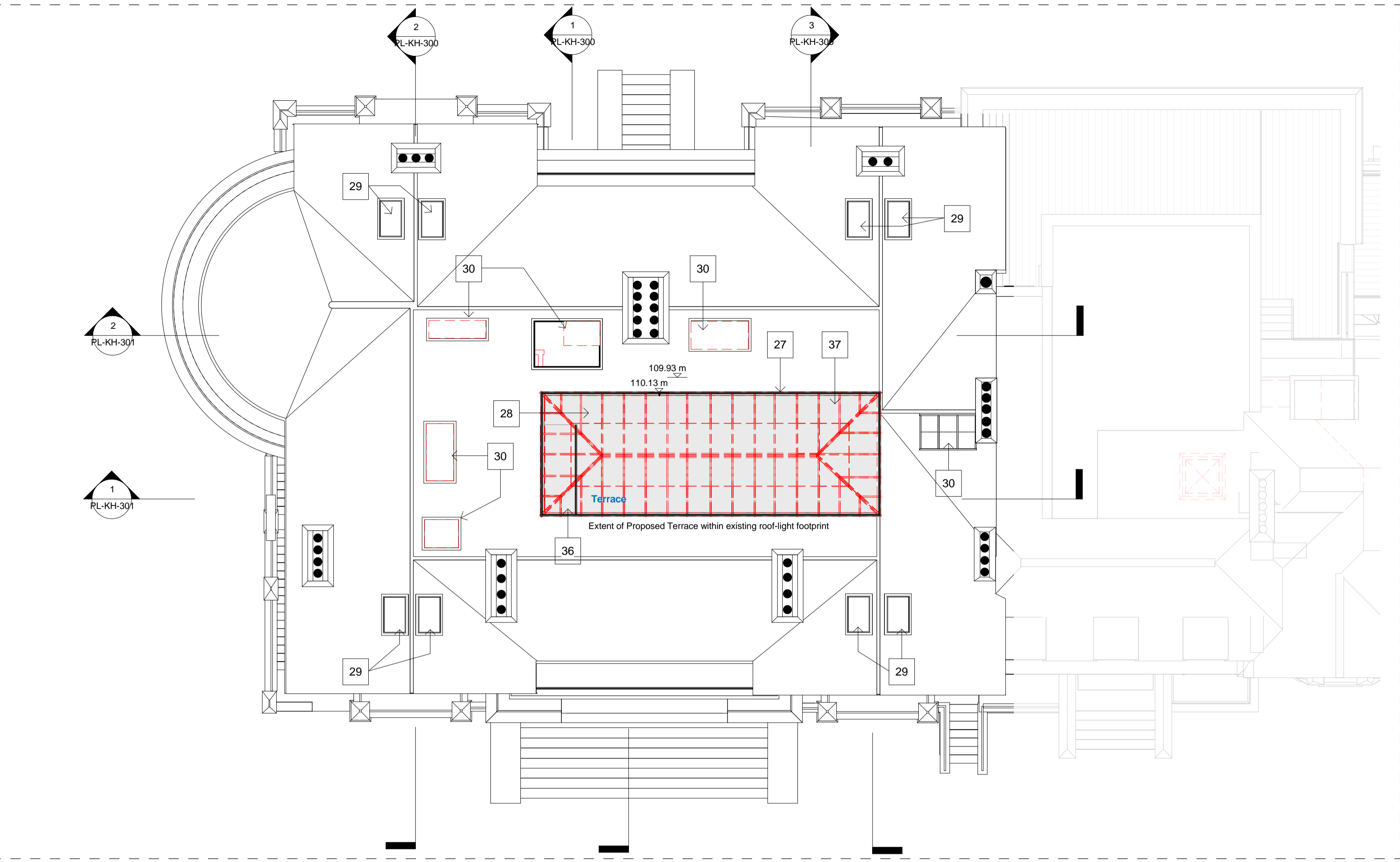
1 Proposed Roof Plan 1 : 100
