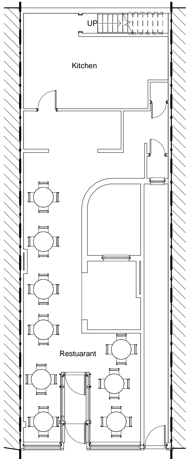
1 Existing Ground Floor. 1 : 100
