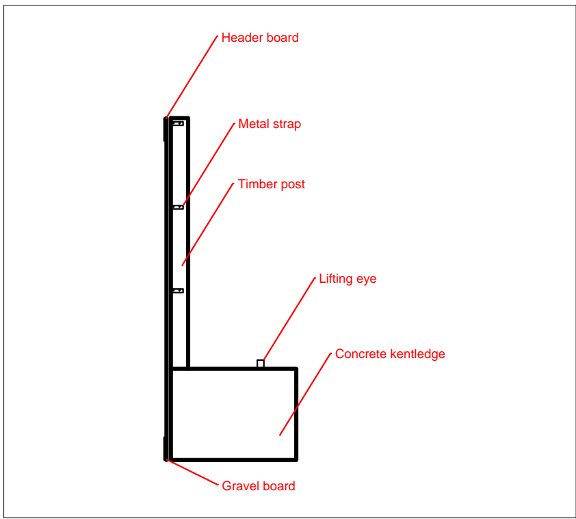
Hoarding - Typical Detail 1 : 20
