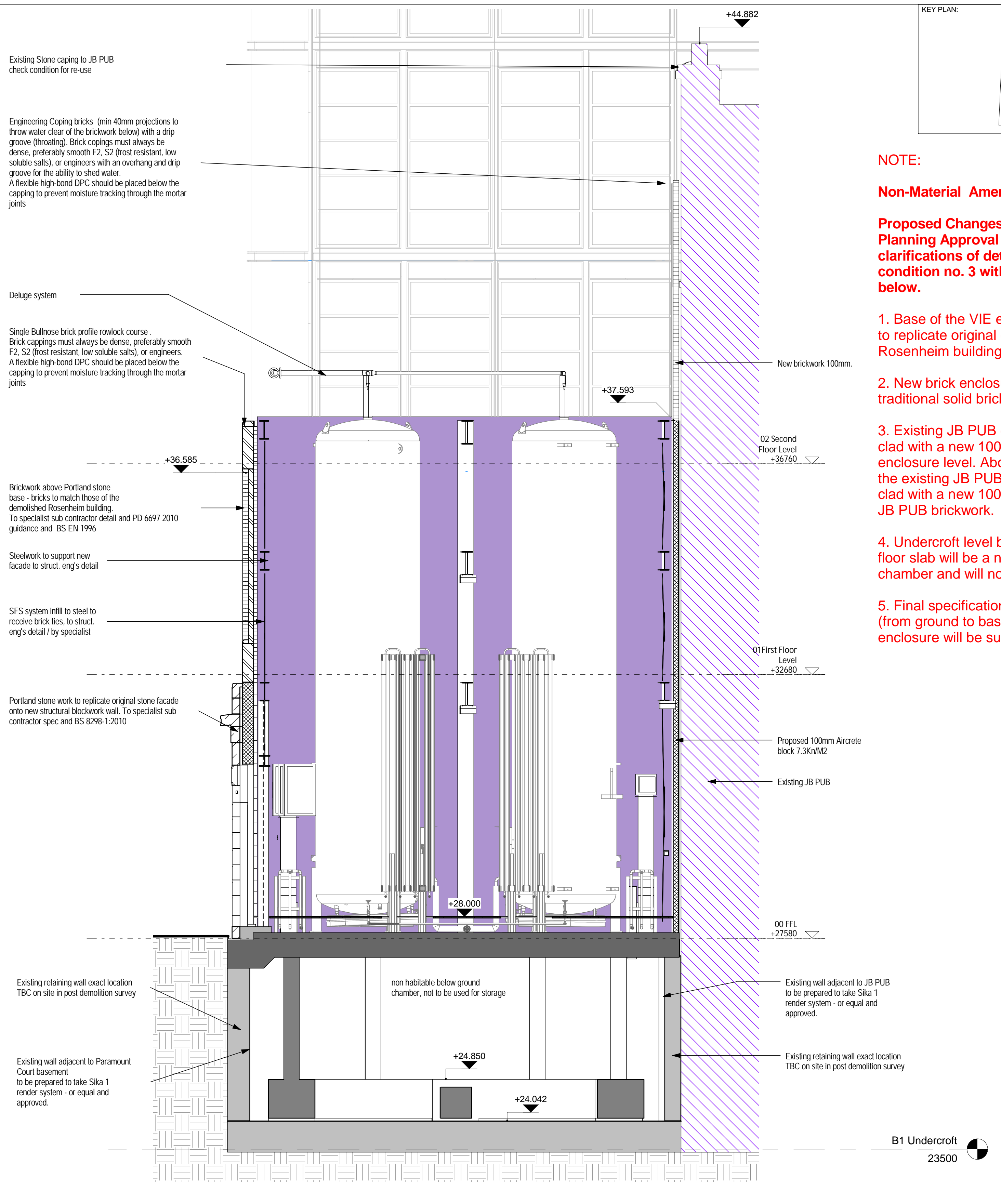
VIE - Long Section 1-50 Non Material Amendment Application
