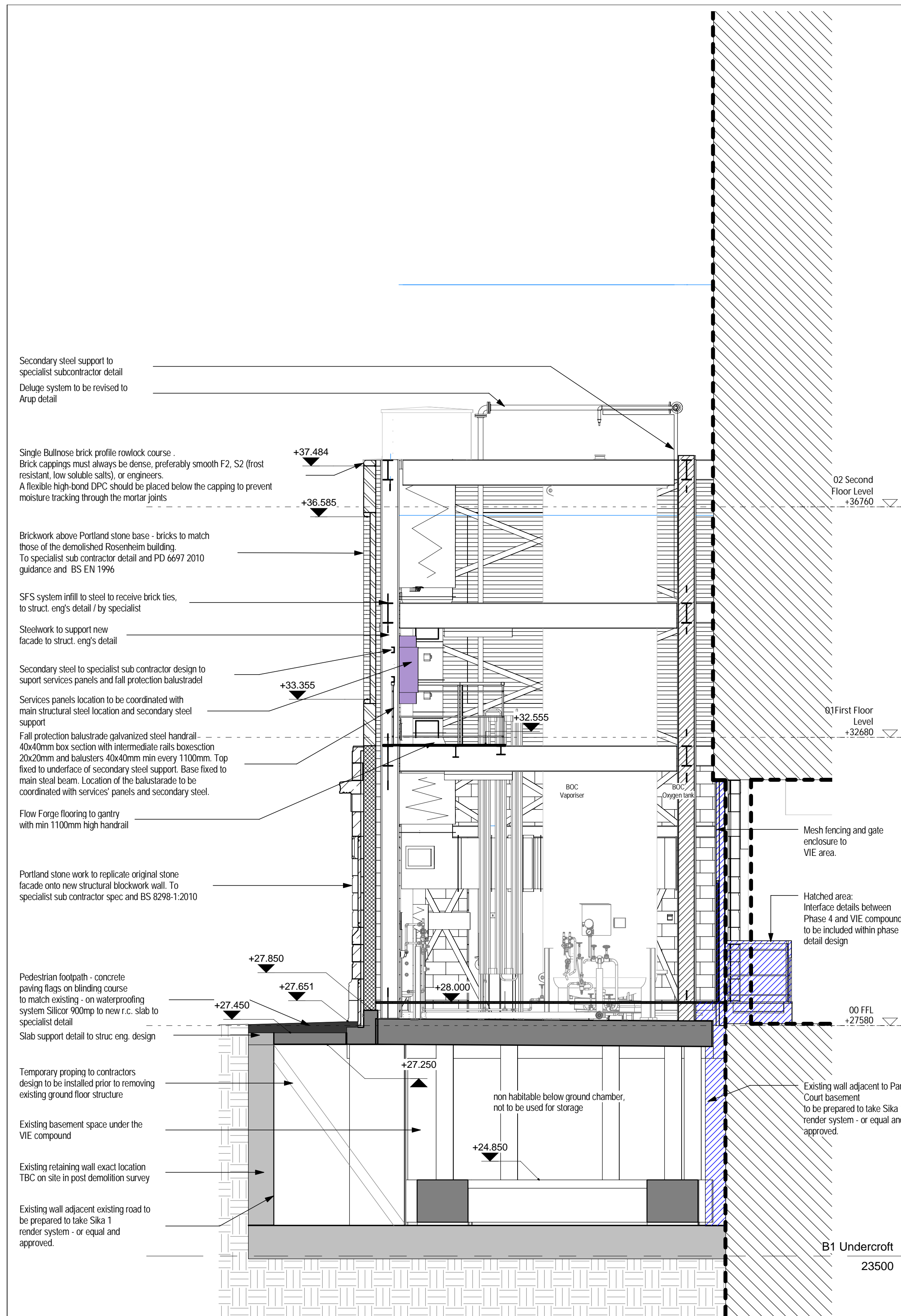
VIE - Cross Section 1-50 Non Material Amendment Application
