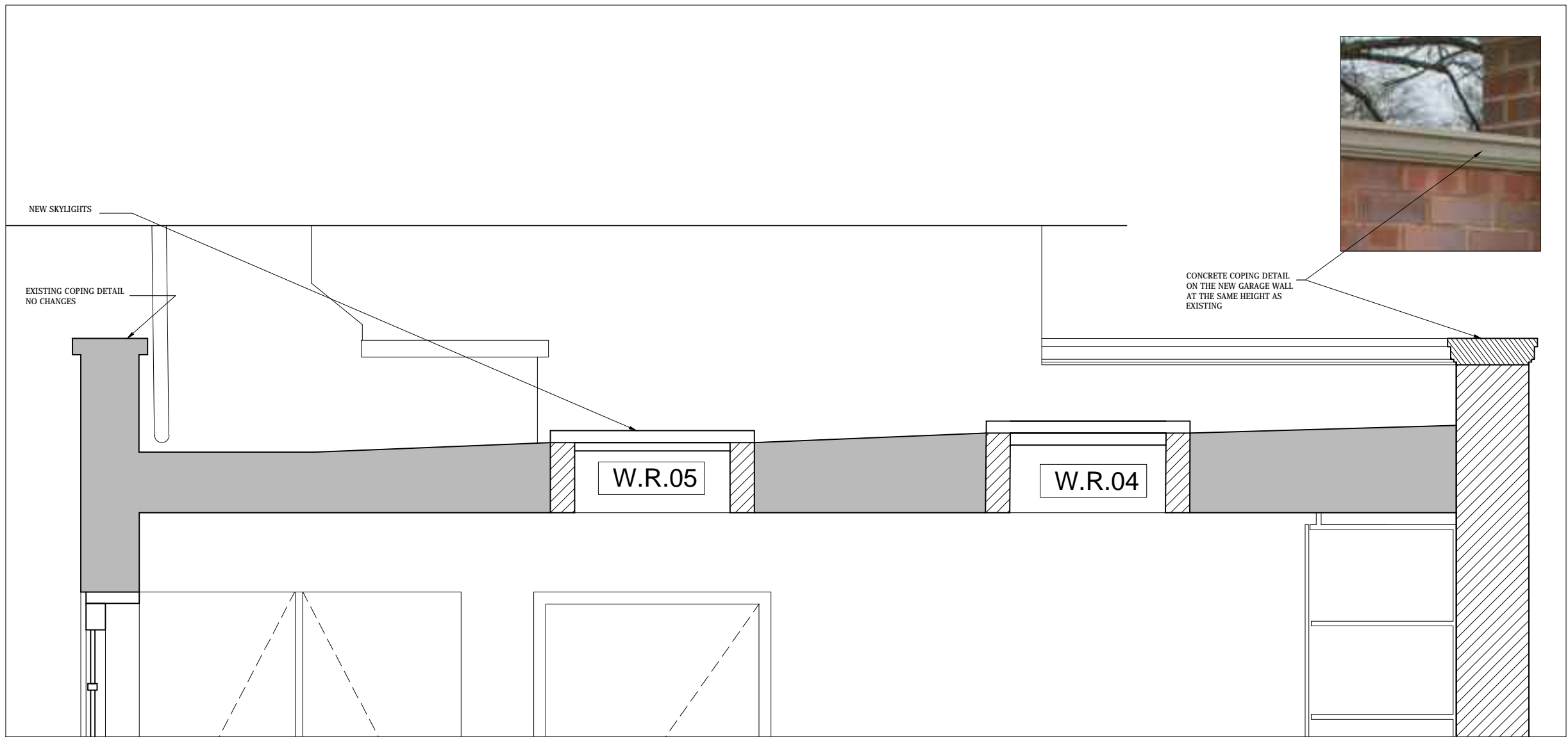
1 GARAGE SECTION 1:10@A1/ 1:20@A3
