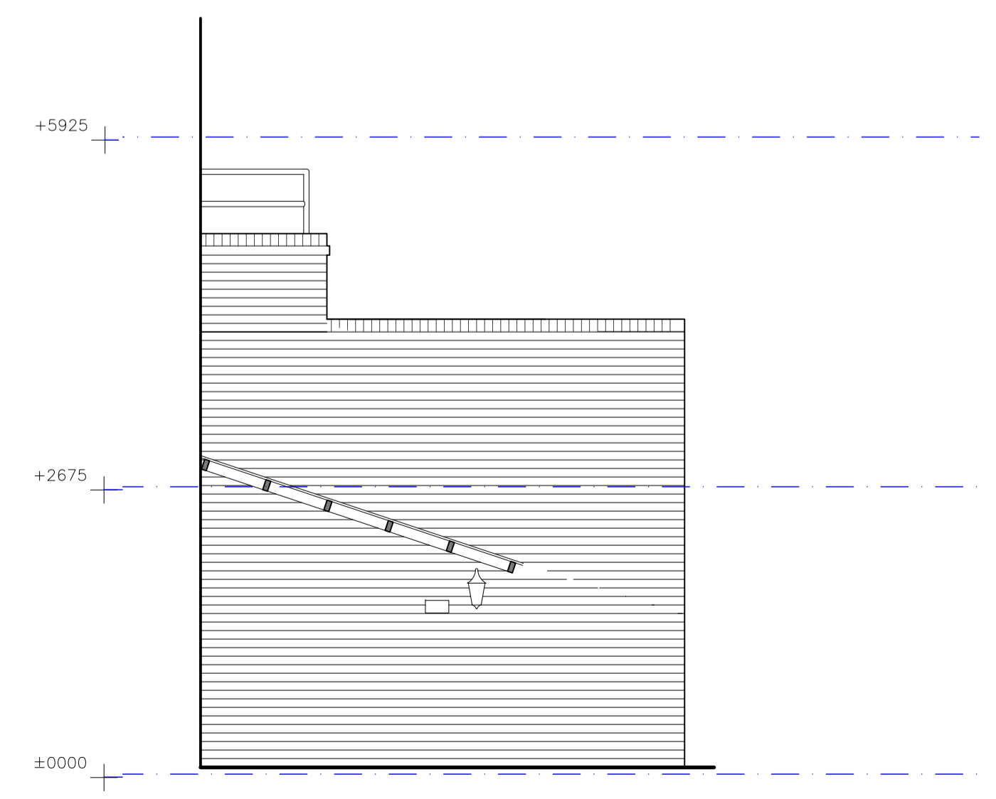
04 West Elevation (Viewed from #152) PROPOSED 1:50
