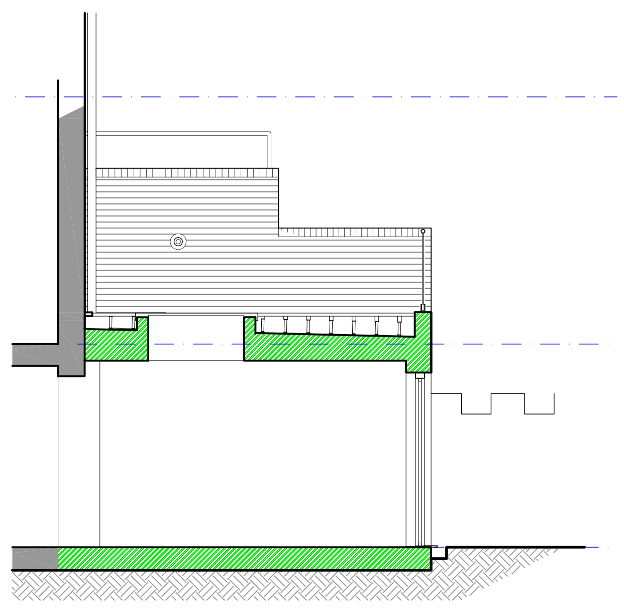
05 West Elevation of East Boundary Wall (Extension #156) PROPOSED 1:50
