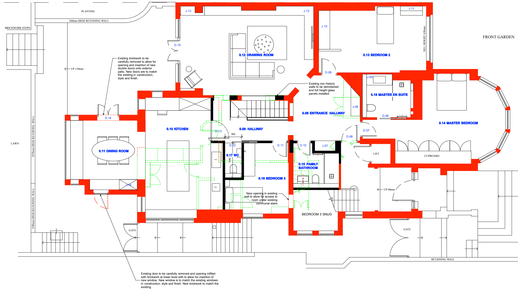
1 PROPOSED GROUND FLOOR PLAN - GIA:164.1 m 2 Scale: 1:50
