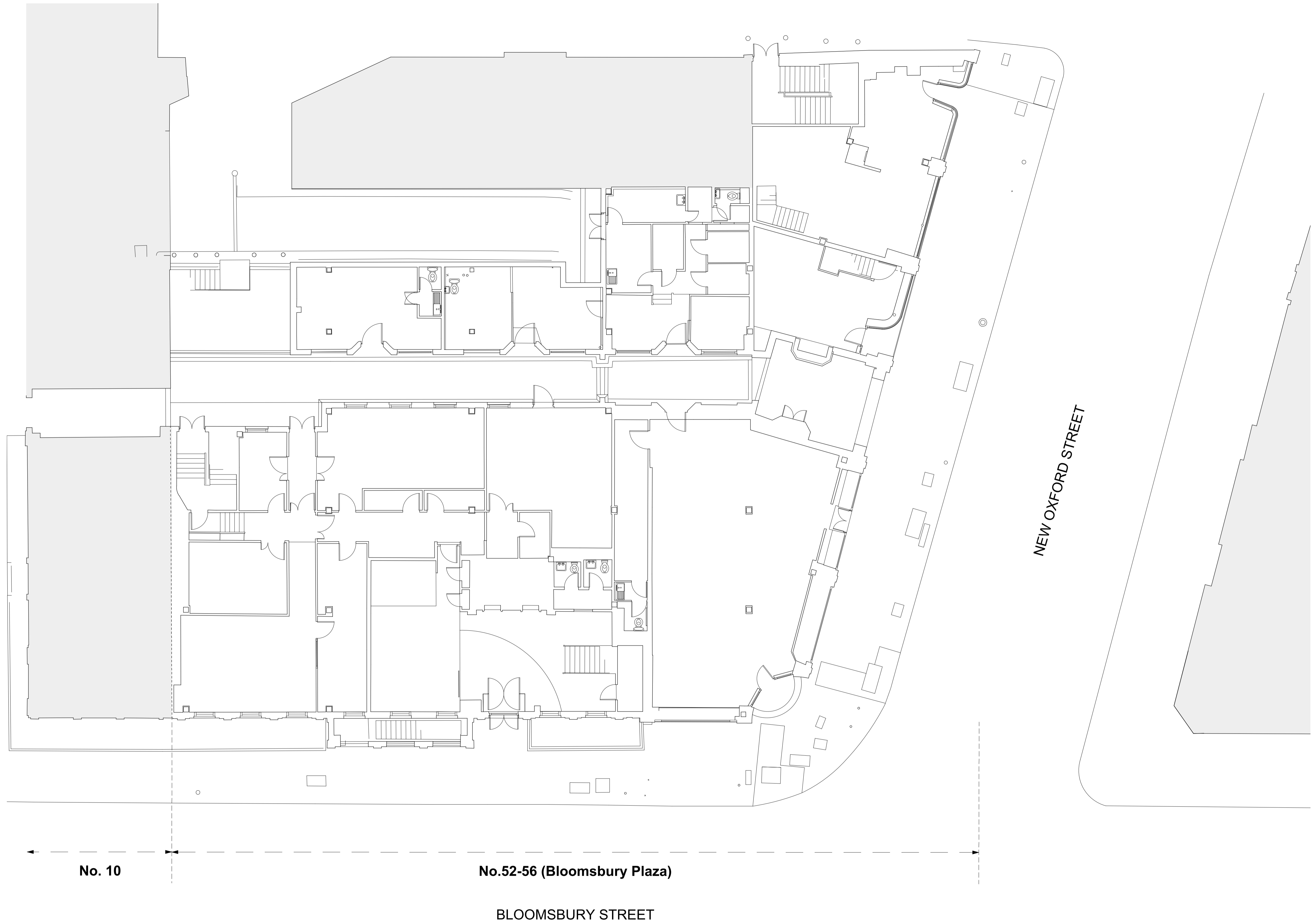
1 Existing Ground Floor Plan 1:100 at A1
