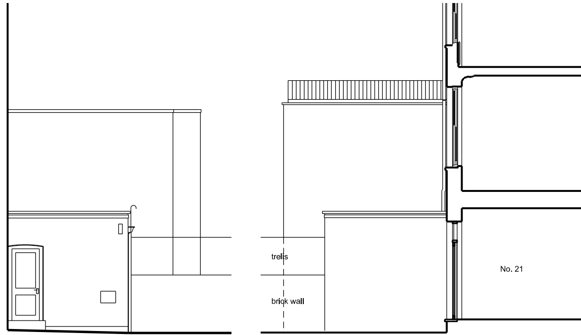
04 Existing South Elevation (part 2) 1:50@ A1 / 1:100@A3
