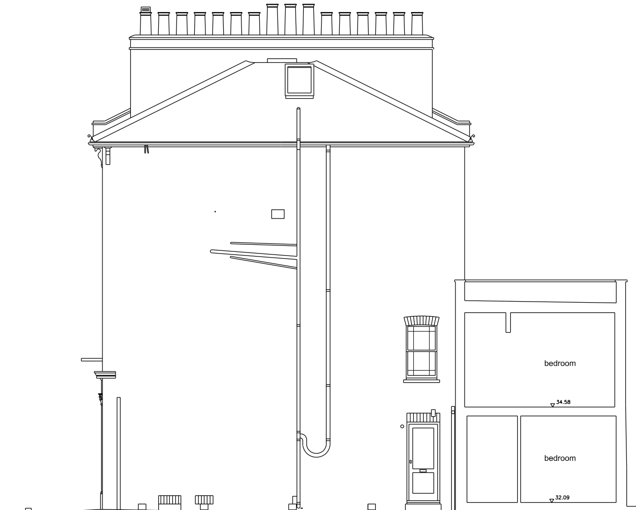
03 Existing South Elevation 1:50@ A1 / 1:100@A3
