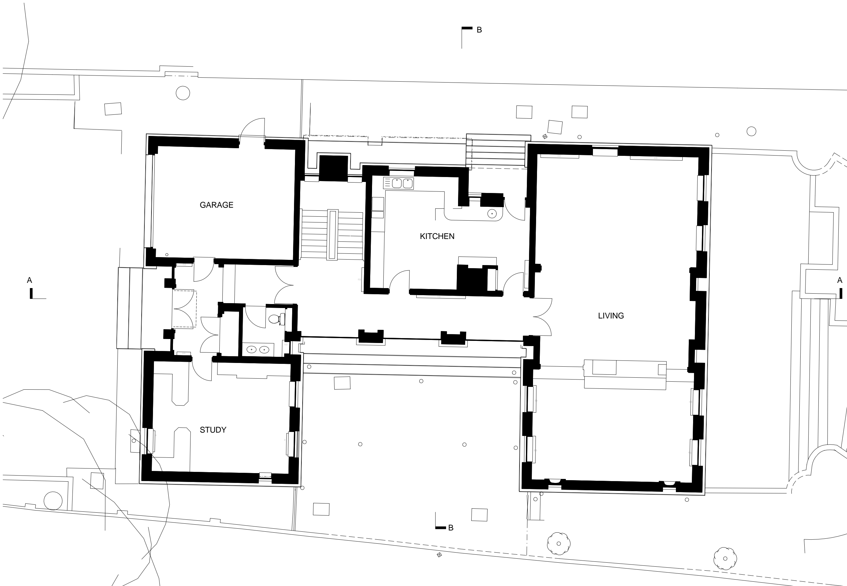
1 EXISTING GROUND FLOOR PLAN
